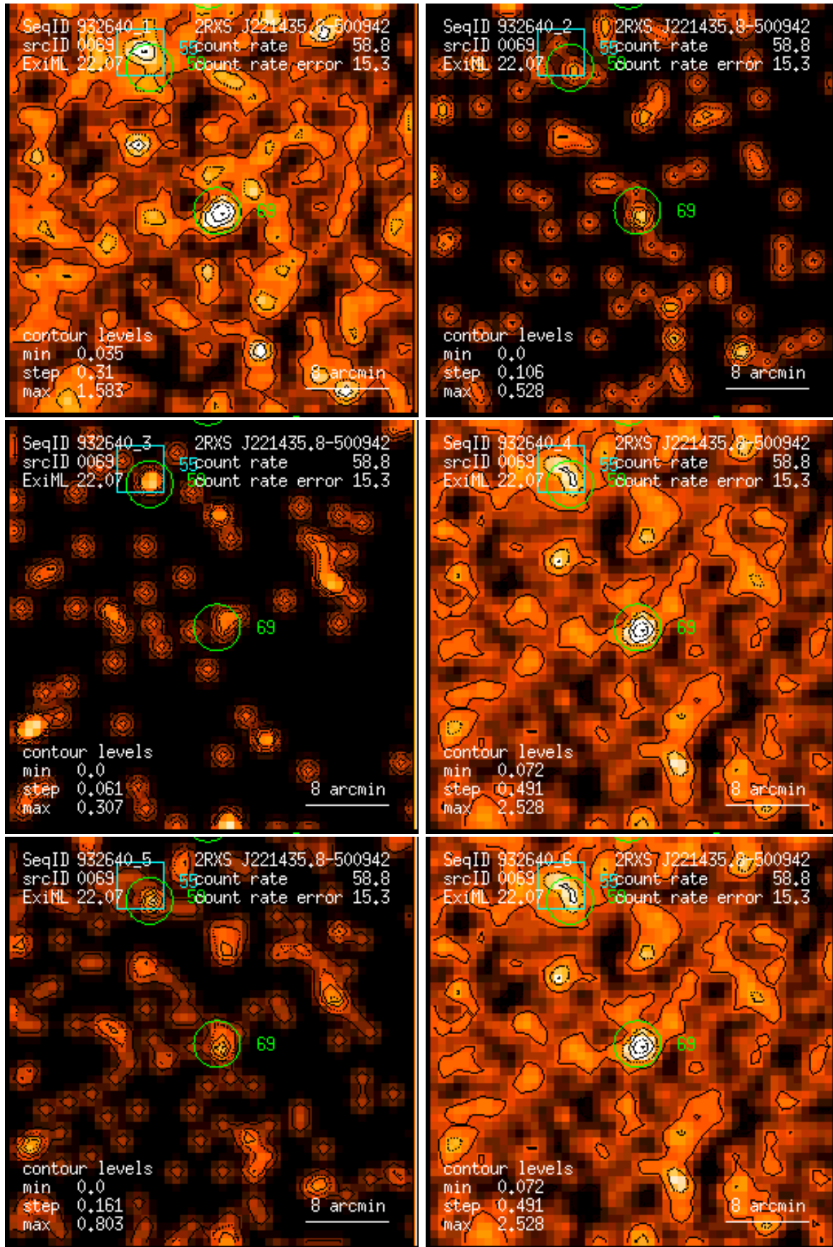
Figure 69: RASS 932640: detection 0069: band rate images, Gaussian filter: (1) PSPC channels 11 – 41, (2) 52 – 90, (3) 91 – 201, (4) 11 – 235, (5) 52 – 201, (6) 11 – 201. Broad band rates in counts/ks. Band rate contour levels in counts/ks/arcmin 2 .
