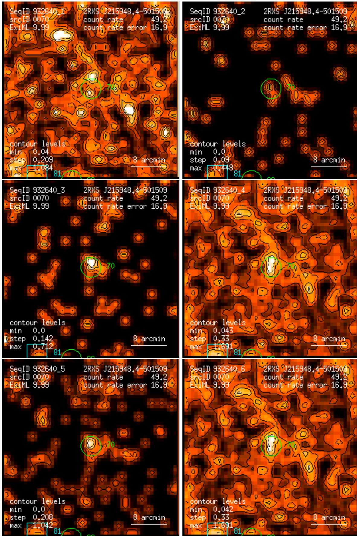
Figure 70: RASS 932640: detection 0070: band rate images, Gaussian filter: (1) PSPC channels 11 – 41, (2) 52 – 90, (3) 91 – 201, (4) 11 – 235, (5) 52 – 201, (6) 11 – 201. Broad band rates in counts/ks. Band rate contour levels in counts/ks/arcmin 2 .
