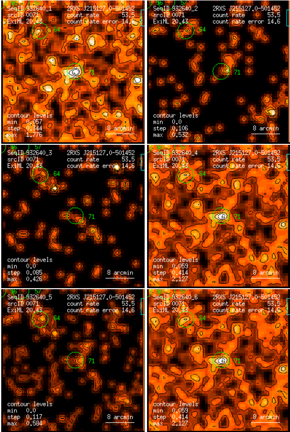
Figure 71: RASS 932640: detection 0071: band rate images, Gaussian filter: (1) PSPC channels 11 – 41, (2) 52 – 90, (3) 91 – 201, (4) 11 – 235, (5) 52 – 201, (6) 11 – 201. Broad band rates in counts/ks. Band rate contour levels in counts/ks/arcmin 2 .
