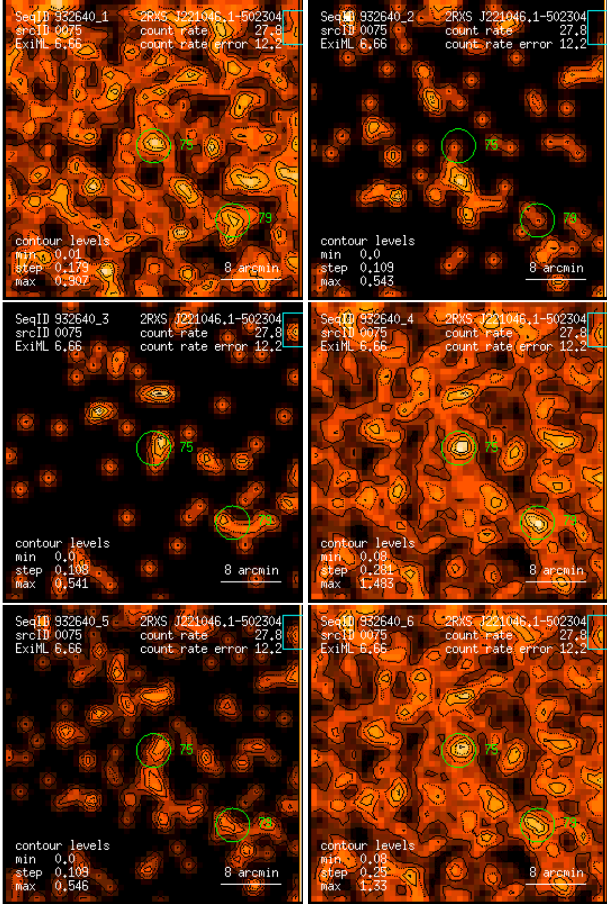
Figure 75: RASS 932640: detection 0075: band rate images, Gaussian filter: (1) PSPC channels 11 – 41, (2) 52 – 90, (3) 91 – 201, (4) 11 – 235, (5) 52 – 201, (6) 11 – 201. Broad band rates in counts/ks. Band rate contour levels in counts/ks/arcmin 2 .
