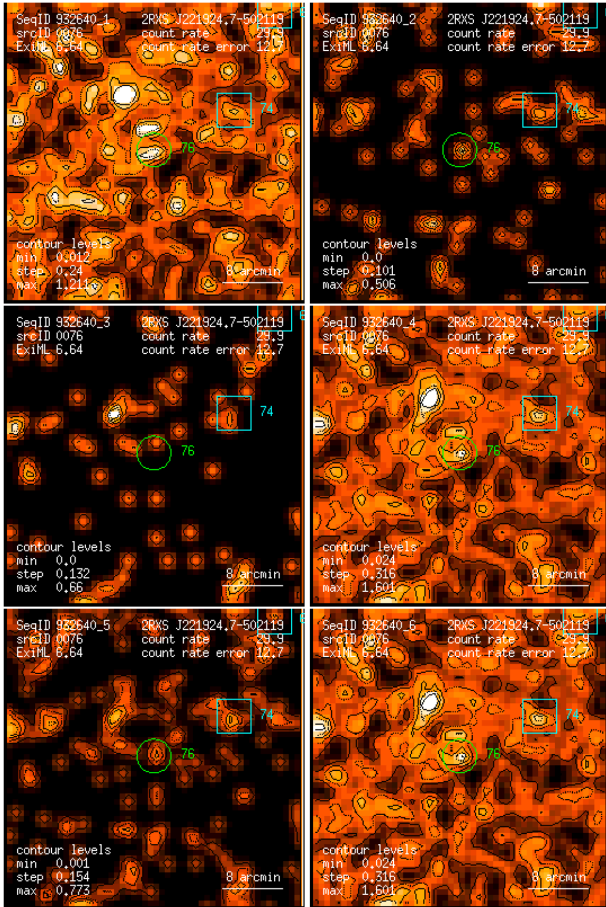
Figure 76: RASS 932640: detection 0076: band rate images, Gaussian filter: (1) PSPC channels 11 – 41, (2) 52 – 90, (3) 91 – 201, (4) 11 – 235, (5) 52 – 201, (6) 11 – 201. Broad band rates in counts/ks. Band rate contour levels in counts/ks/arcmin 2 .
