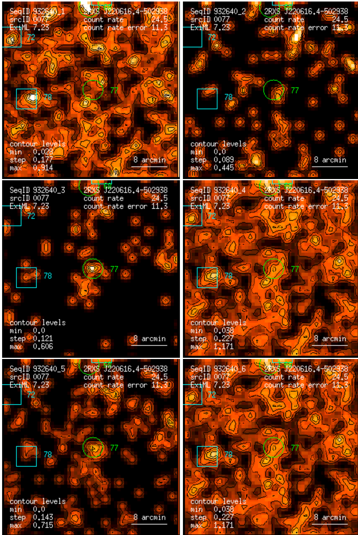
Figure 77: RASS 932640: detection 0077: band rate images, Gaussian filter: (1) PSPC channels 11 – 41, (2) 52 – 90, (3) 91 – 201, (4) 11 – 235, (5) 52 – 201, (6) 11 – 201. Broad band rates in counts/ks. Band rate contour levels in counts/ks/arcmin 2 .
