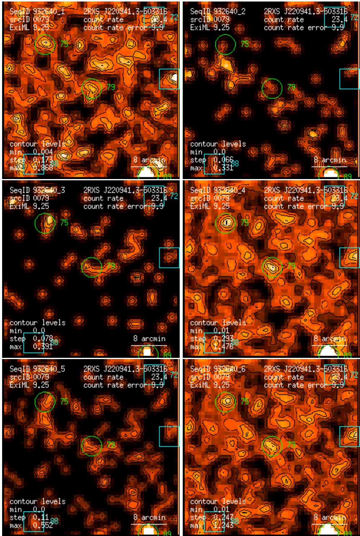
Figure 79: RASS 932640: detection 0079: band rate images, Gaussian filter: (1) PSPC channels 11 – 41, (2) 52 – 90, (3) 91 – 201, (4) 11 – 235, (5) 52 – 201, (6) 11 – 201. Broad band rates in counts/ks. Band rate contour levels in counts/ks/arcmin 2 .
