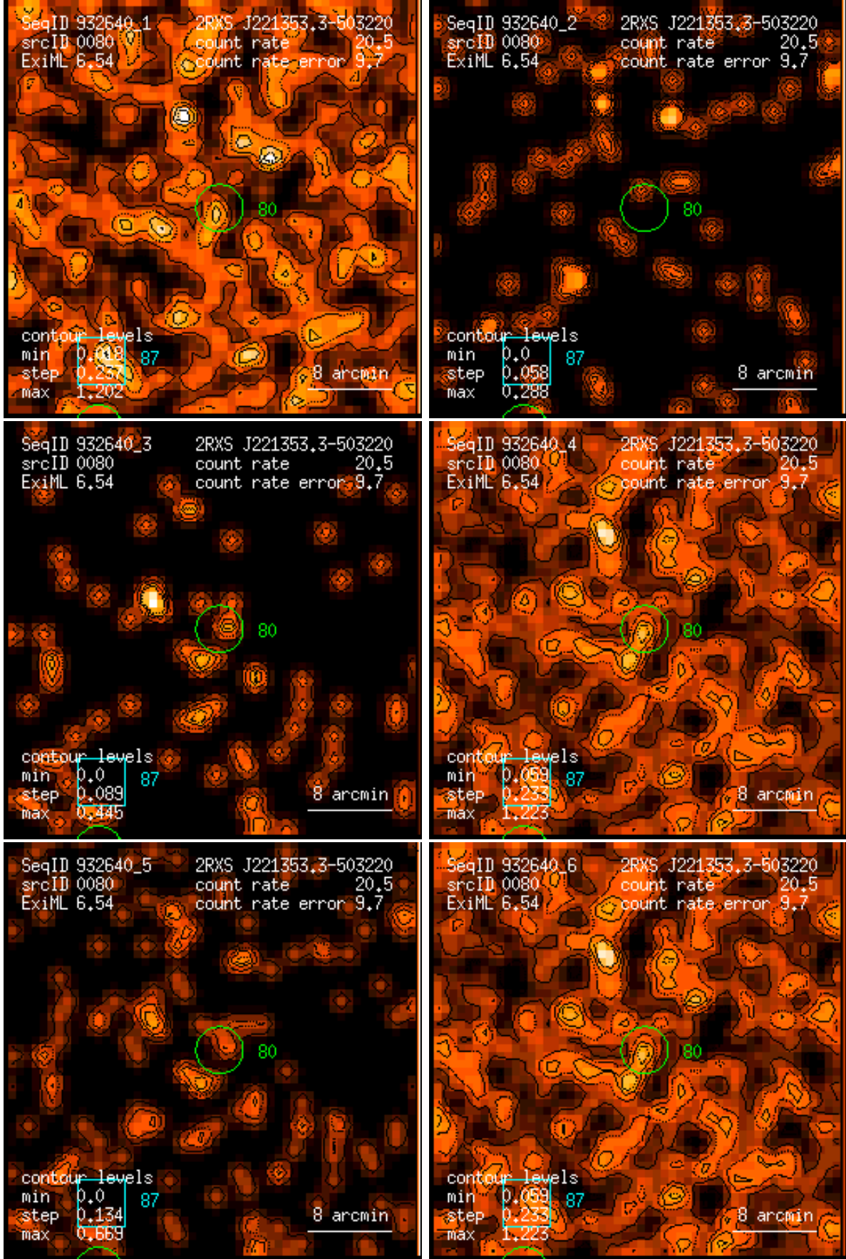
Figure 80: RASS 932640: detection 0080: band rate images, Gaussian filter: (1) PSPC channels 11 – 41, (2) 52 – 90, (3) 91 – 201, (4) 11 – 235, (5) 52 – 201, (6) 11 – 201. Broad band rates in counts/ks. Band rate contour levels in counts/ks/arcmin 2 .
