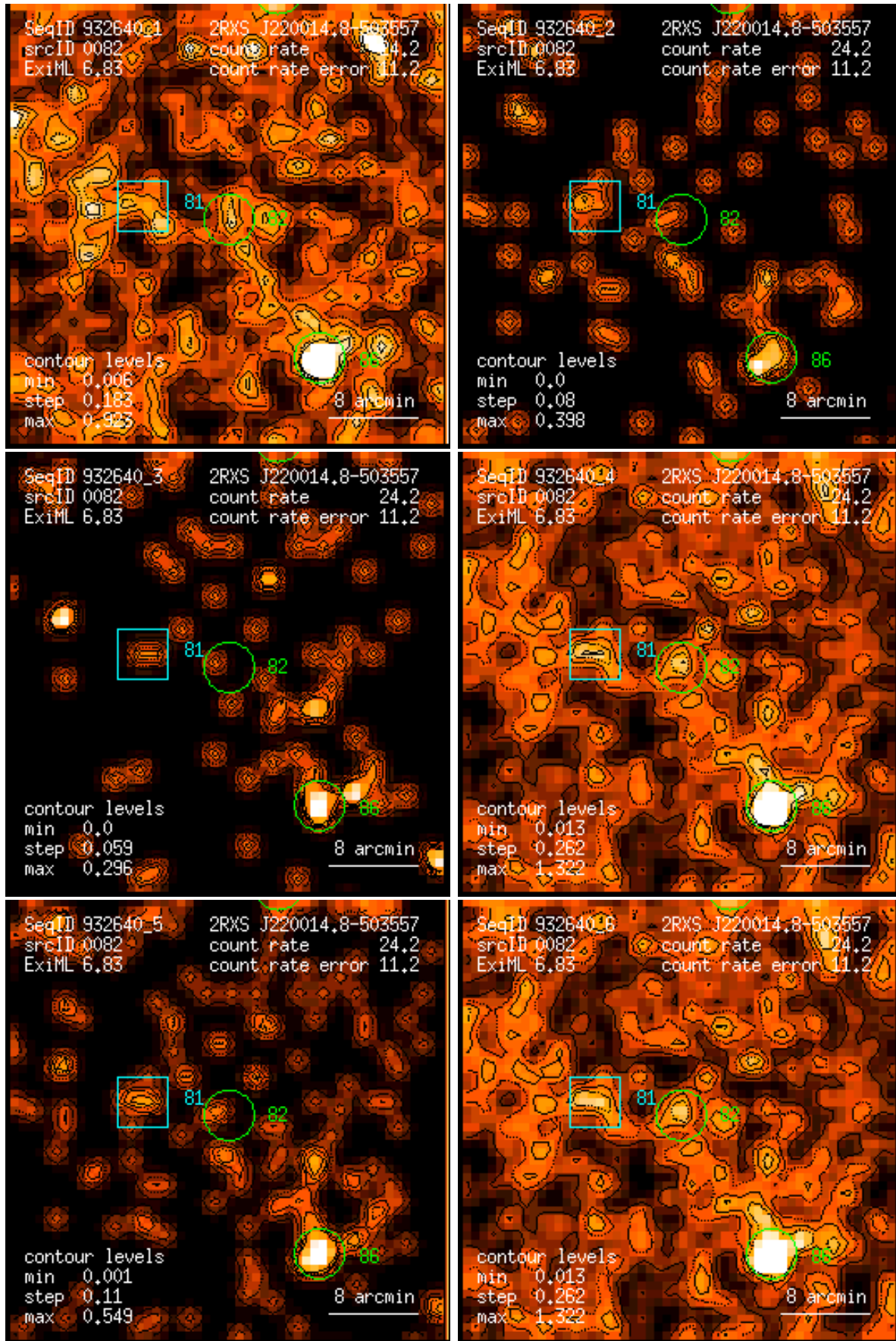
Figure 82: RASS 932640: detection 0082: band rate images, Gaussian filter: (1) PSPC channels 11 – 41, (2) 52 – 90, (3) 91 – 201, (4) 11 – 235, (5) 52 – 201, (6) 11 – 201. Broad band rates in counts/ks. Band rate contour levels in counts/ks/arcmin 2 .
