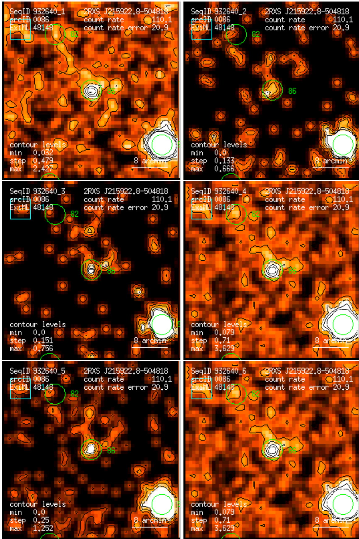
Figure 86: RASS 932640: detection 0086: band rate images, Gaussian filter: (1) PSPC channels 11 – 41, (2) 52 – 90, (3) 91 – 201, (4) 11 – 235, (5) 52 – 201, (6) 11 – 201. Broad band rates in counts/ks. Band rate contour levels in counts/ks/arcmin 2 .
