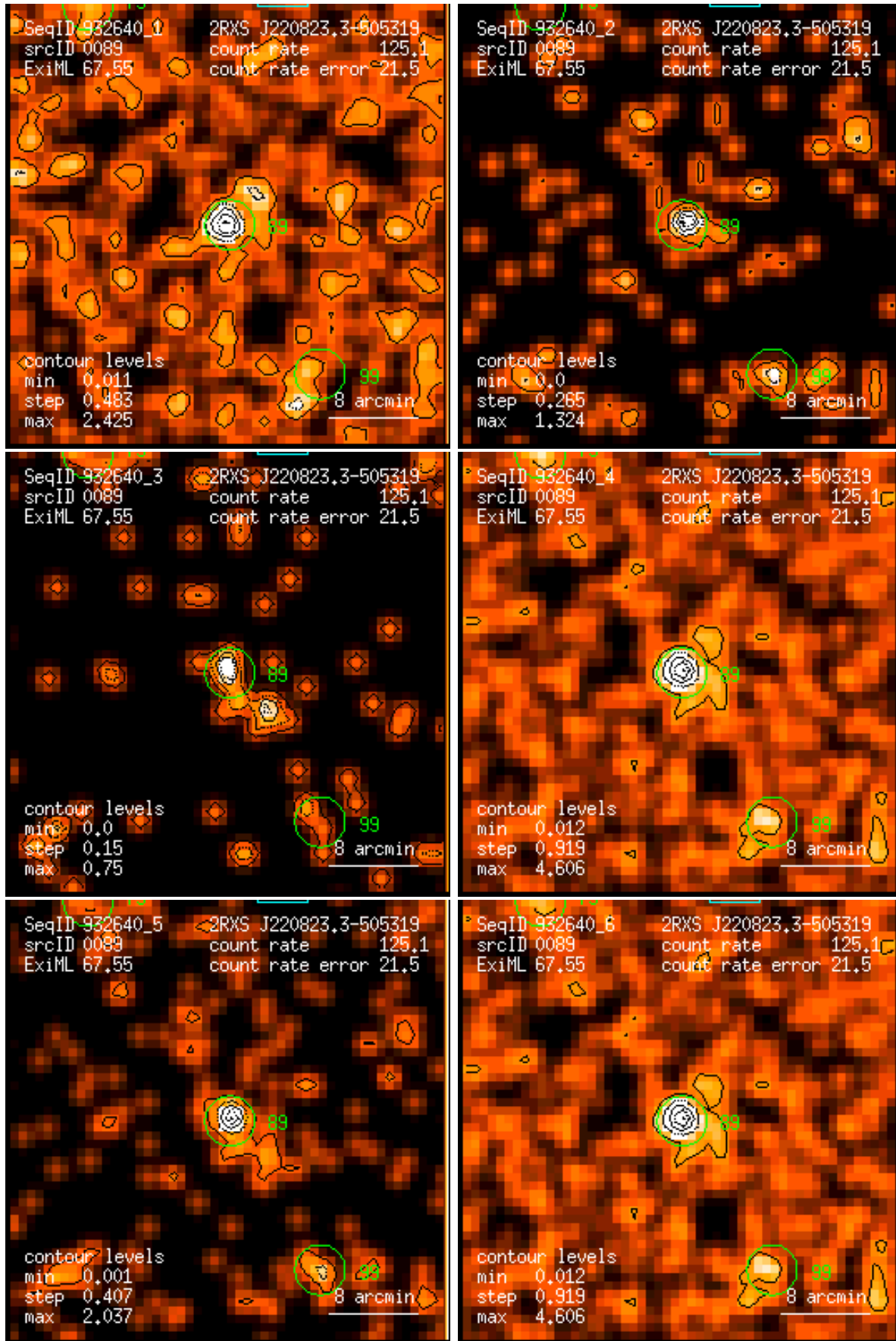
Figure 89: RASS 932640: detection 0089: band rate images, Gaussian filter: (1) PSPC channels 11 – 41, (2) 52 – 90, (3) 91 – 201, (4) 11 – 235, (5) 52 – 201, (6) 11 – 201. Broad band rates in counts/ks. Band rate contour levels in counts/ks/arcmin 2 .
