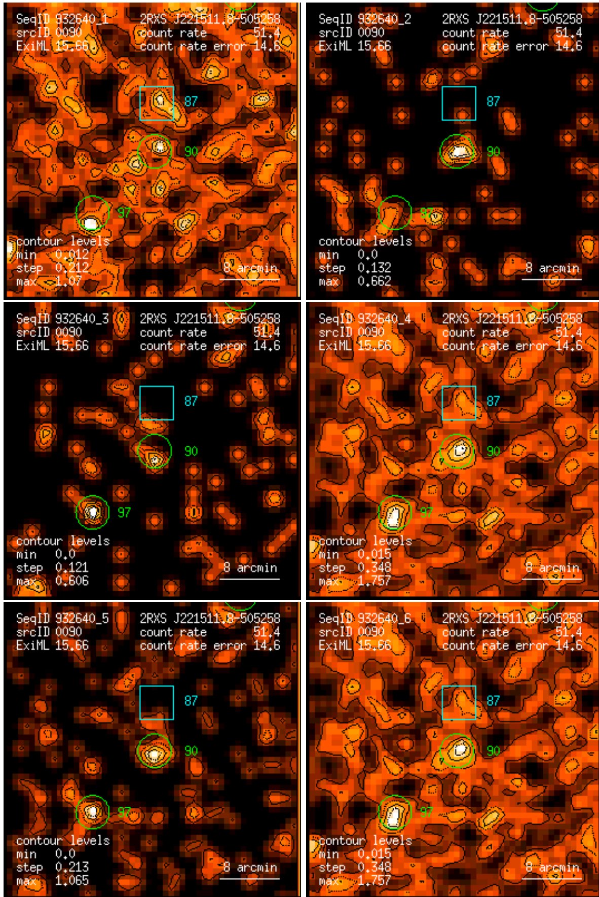
Figure 90: RASS 932640: detection 0090: band rate images, Gaussian filter: (1) PSPC channels 11 – 41, (2) 52 – 90, (3) 91 – 201, (4) 11 – 235, (5) 52 – 201, (6) 11 – 201. Broad band rates in counts/ks. Band rate contour levels in counts/ks/arcmin 2 .
