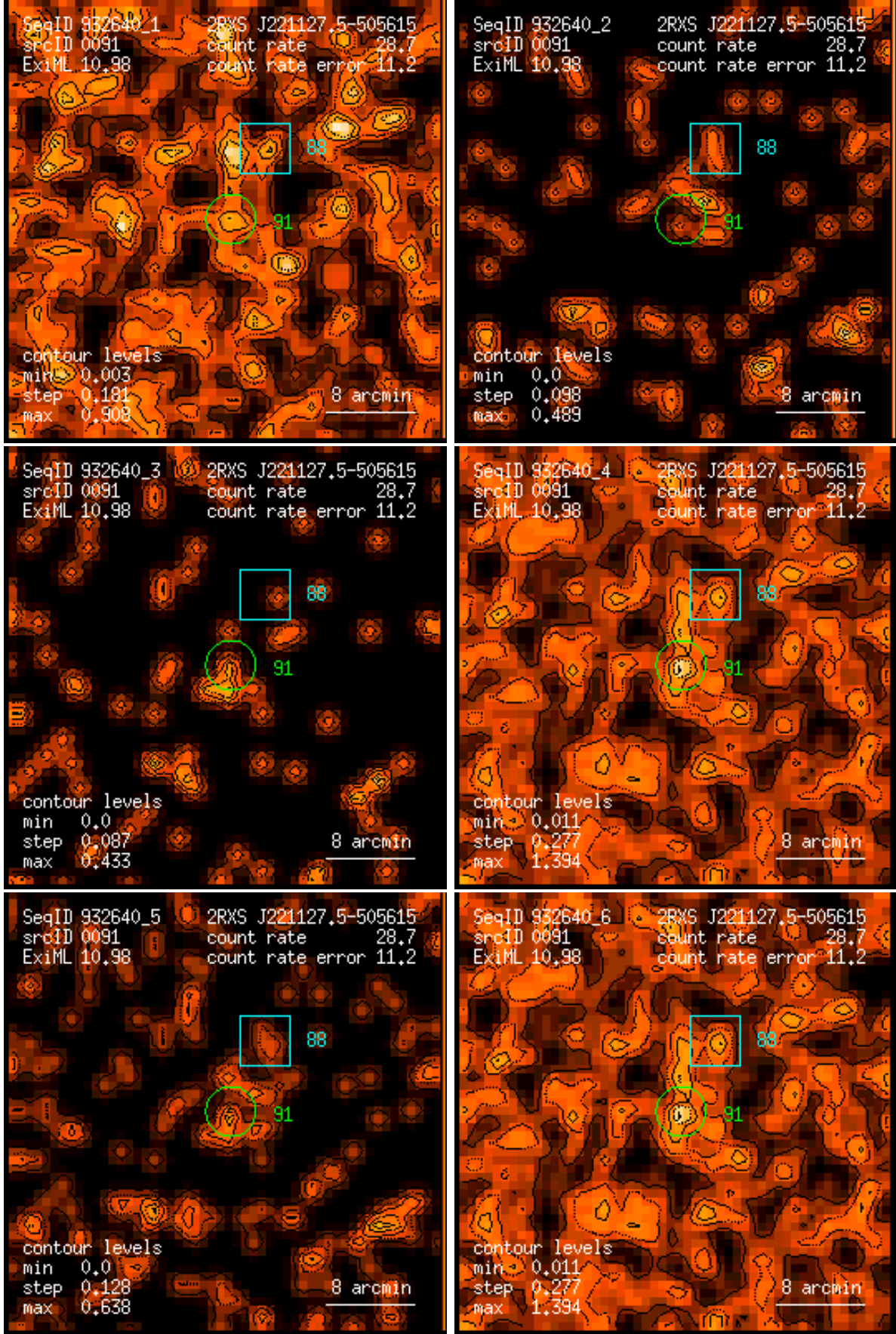
Figure 91: RASS 932640: detection 0091: band rate images, Gaussian filter: (1) PSPC channels 11 – 41, (2) 52 – 90, (3) 91 – 201, (4) 11 – 235, (5) 52 – 201, (6) 11 – 201. Broad band rates in counts/ks. Band rate contour levels in counts/ks/arcmin 2 .
