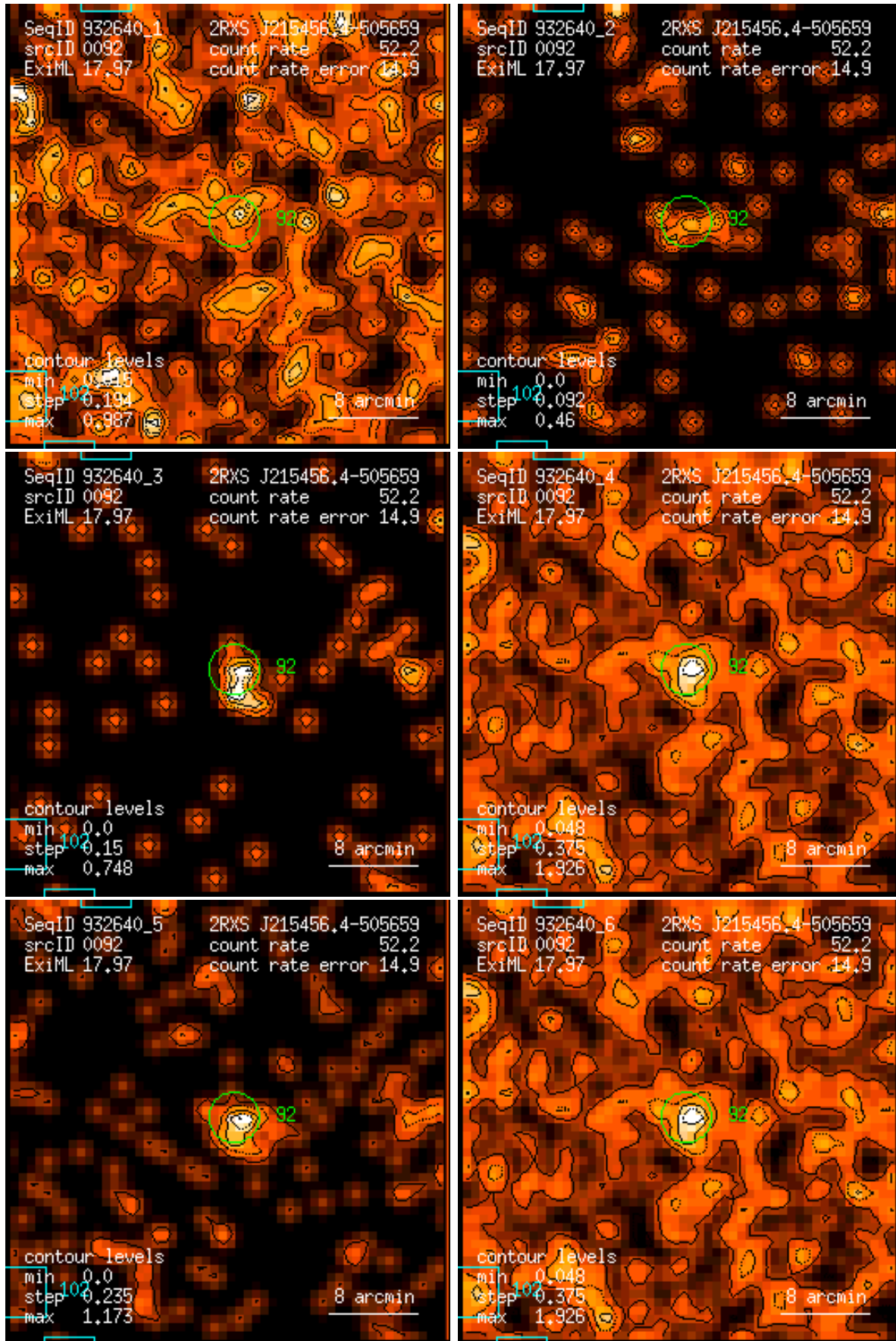
Figure 92: RASS 932640: detection 0092: band rate images, Gaussian filter: (1) PSPC channels 11 – 41, (2) 52 – 90, (3) 91 – 201, (4) 11 – 235, (5) 52 – 201, (6) 11 – 201. Broad band rates in counts/ks. Band rate contour levels in counts/ks/arcmin 2 .
