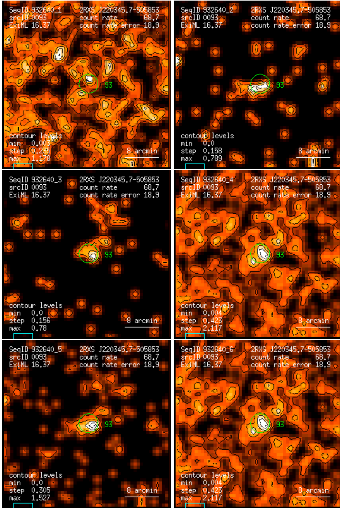
Figure 93: RASS 932640: detection 0093: band rate images, Gaussian filter: (1) PSPC channels 11 – 41, (2) 52 – 90, (3) 91 – 201, (4) 11 – 235, (5) 52 – 201, (6) 11 – 201. Broad band rates in counts/ks. Band rate contour levels in counts/ks/arcmin 2 .
