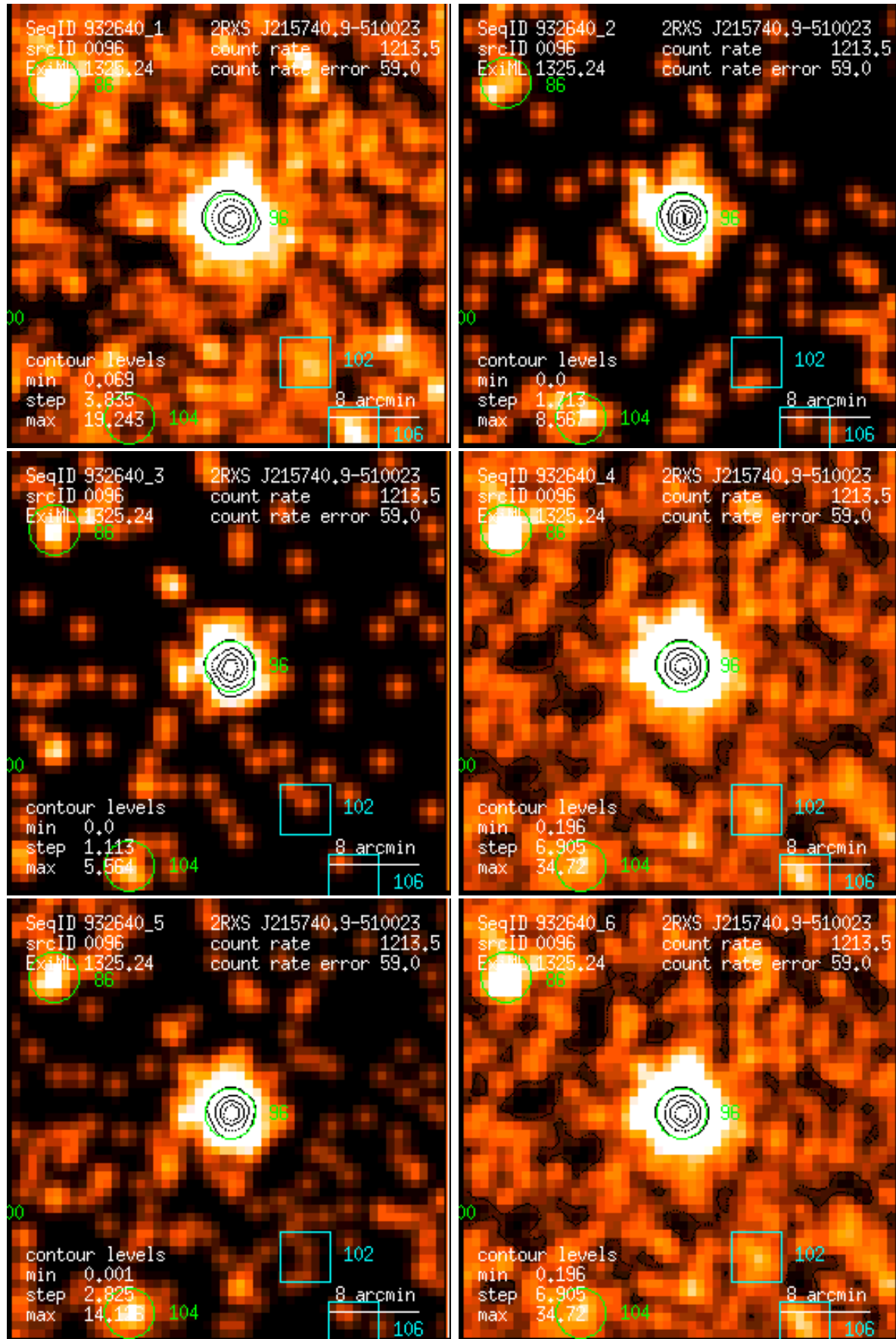
Figure 96: RASS 932640: detection 0096: band rate images, Gaussian filter: (1) PSPC channels 11 – 41, (2) 52 – 90, (3) 91 – 201, (4) 11 – 235, (5) 52 – 201, (6) 11 – 201. Broad band rates in counts/ks. Band rate contour levels in counts/ks/arcmin 2 .
