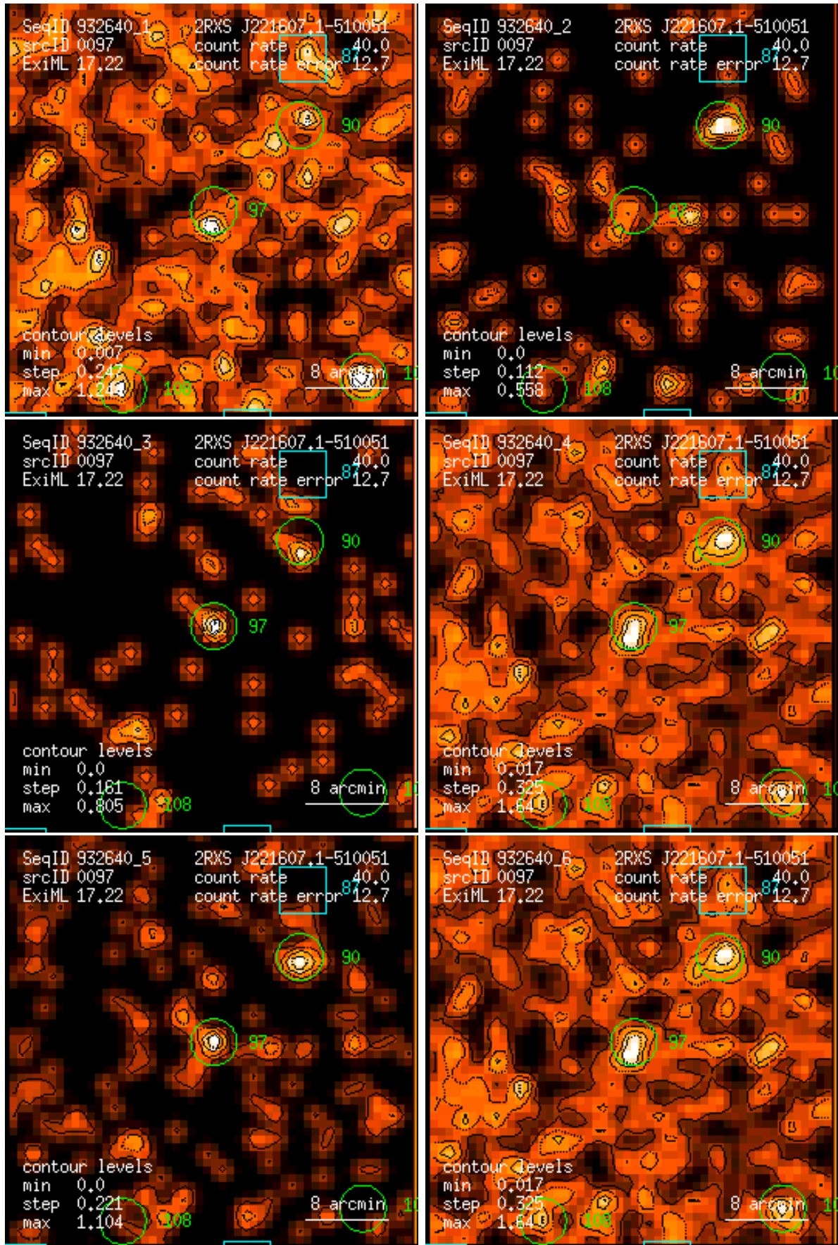
Figure 97: RASS 932640: detection 0097: band rate images, Gaussian filter: (1) PSPC channels 11 – 41, (2) 52 – 90, (3) 91 – 201, (4) 11 – 235, (5) 52 – 201, (6) 11 – 201. Broad band rates in counts/ks. Band rate contour levels in counts/ks/arcmin 2 .
