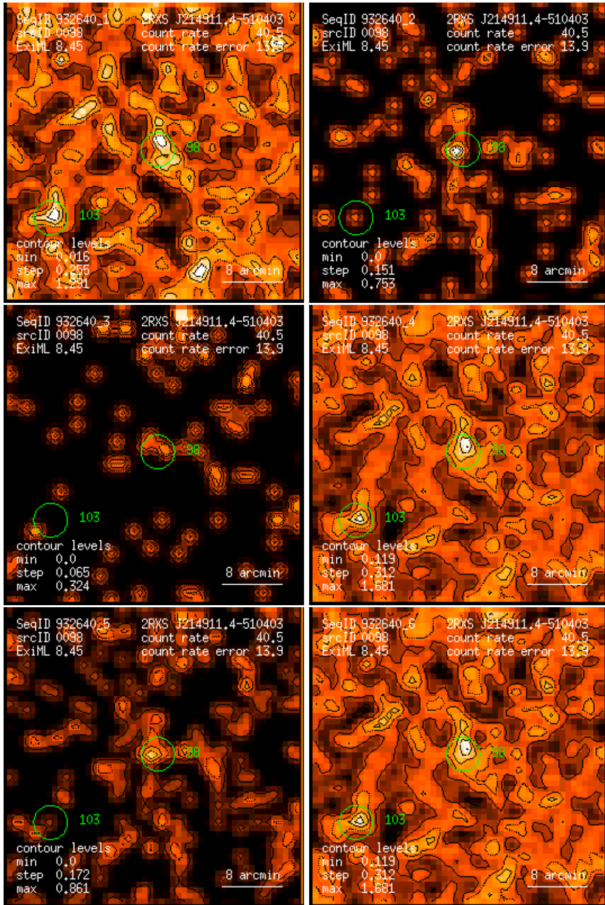
Figure 98: RASS 932640: detection 0098: band rate images, Gaussian filter: (1) PSPC channels 11 – 41, (2) 52 – 90, (3) 91 – 201, (4) 11 – 235, (5) 52 – 201, (6) 11 – 201. Broad band rates in counts/ks. Band rate contour levels in counts/ks/arcmin 2 .
