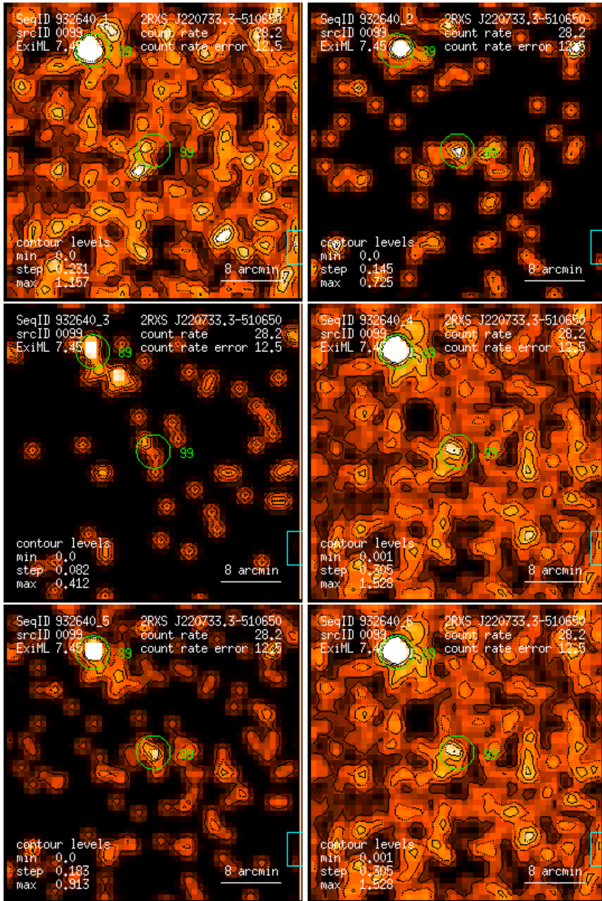
Figure 99: RASS 932640: detection 0099: band rate images, Gaussian filter: (1) PSPC channels 11 – 41, (2) 52 – 90, (3) 91 – 201, (4) 11 – 235, (5) 52 – 201, (6) 11 – 201. Broad band rates in counts/ks. Band rate contour levels in counts/ks/arcmin 2 .
