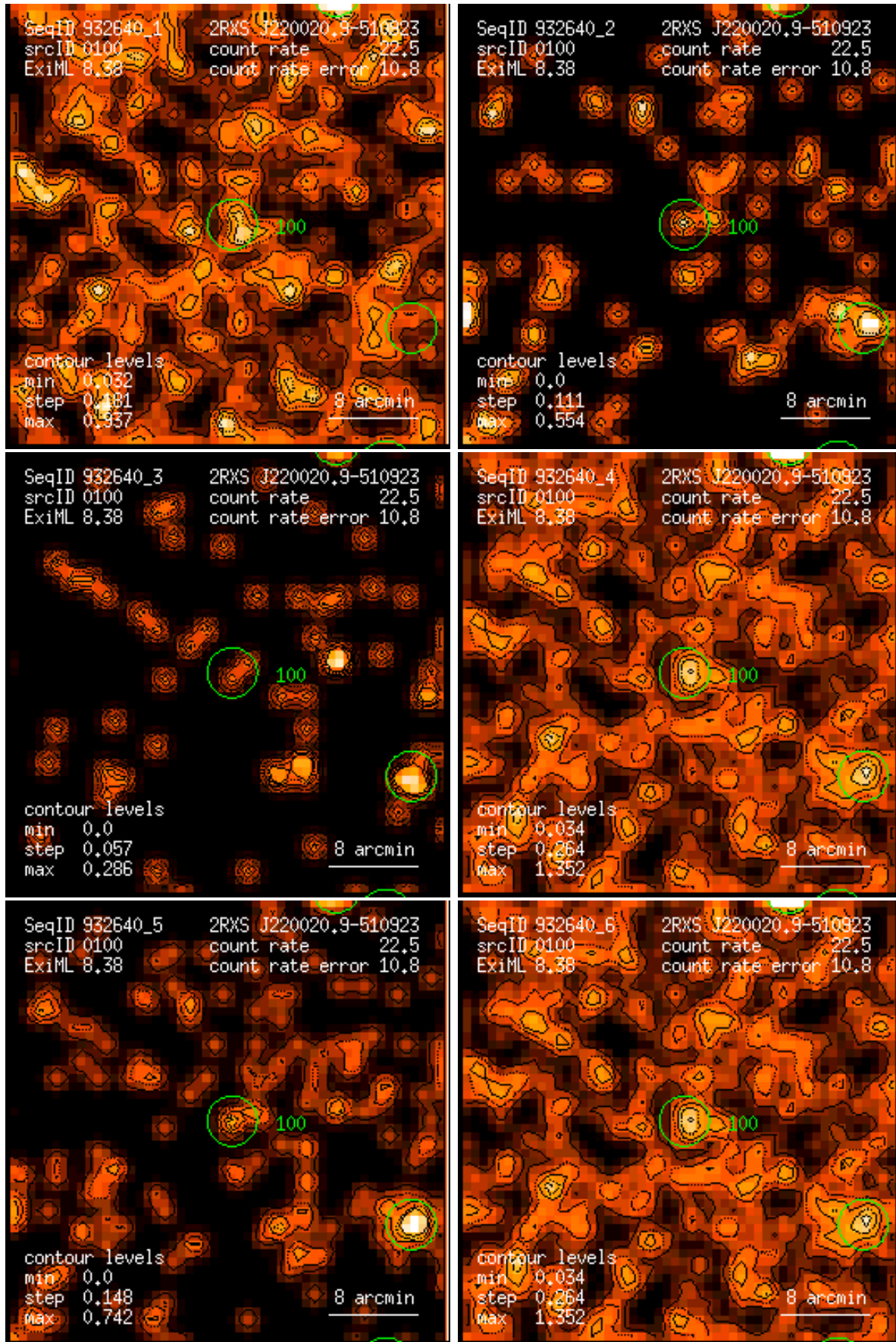
Figure 100: RASS 932640: detection 0100: band rate images, Gaussian filter: (1) PSPC channels 11 – 41, (2) 52 – 90, (3) 91 – 201, (4) 11 – 235, (5) 52 – 201, (6) 11 – 201. Broad band rates in counts/ks. Band rate contour levels in counts/ks/arcmin 2 .
