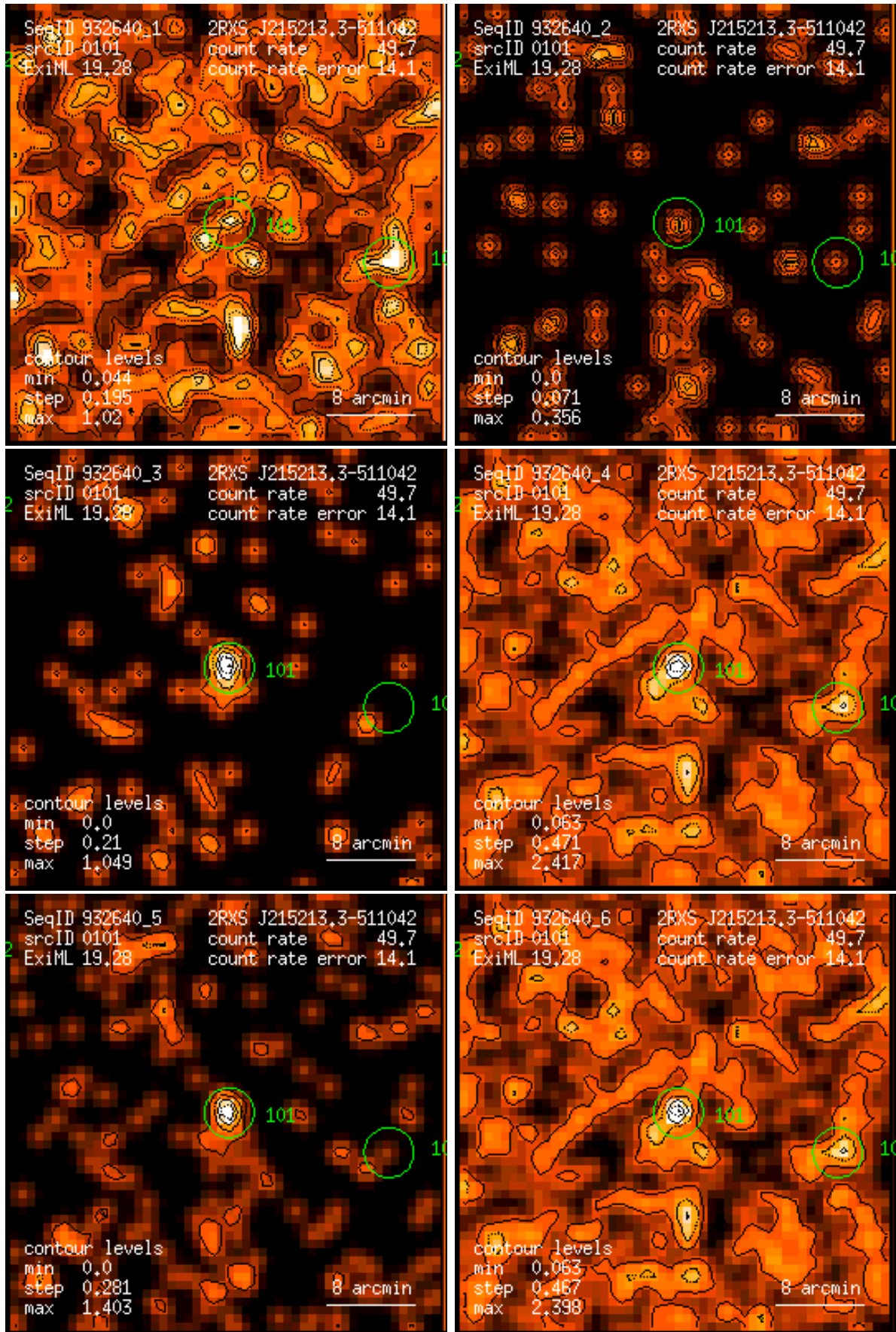
Figure 101: RASS 932640: detection 0101: band rate images, Gaussian filter: (1) PSPC channels 11 – 41, (2) 52 – 90, (3) 91 – 201, (4) 11 – 235, (5) 52 – 201, (6) 11 – 201. Broad band rates in counts/ks. Band rate contour levels in counts/ks/arcmin 2 .
