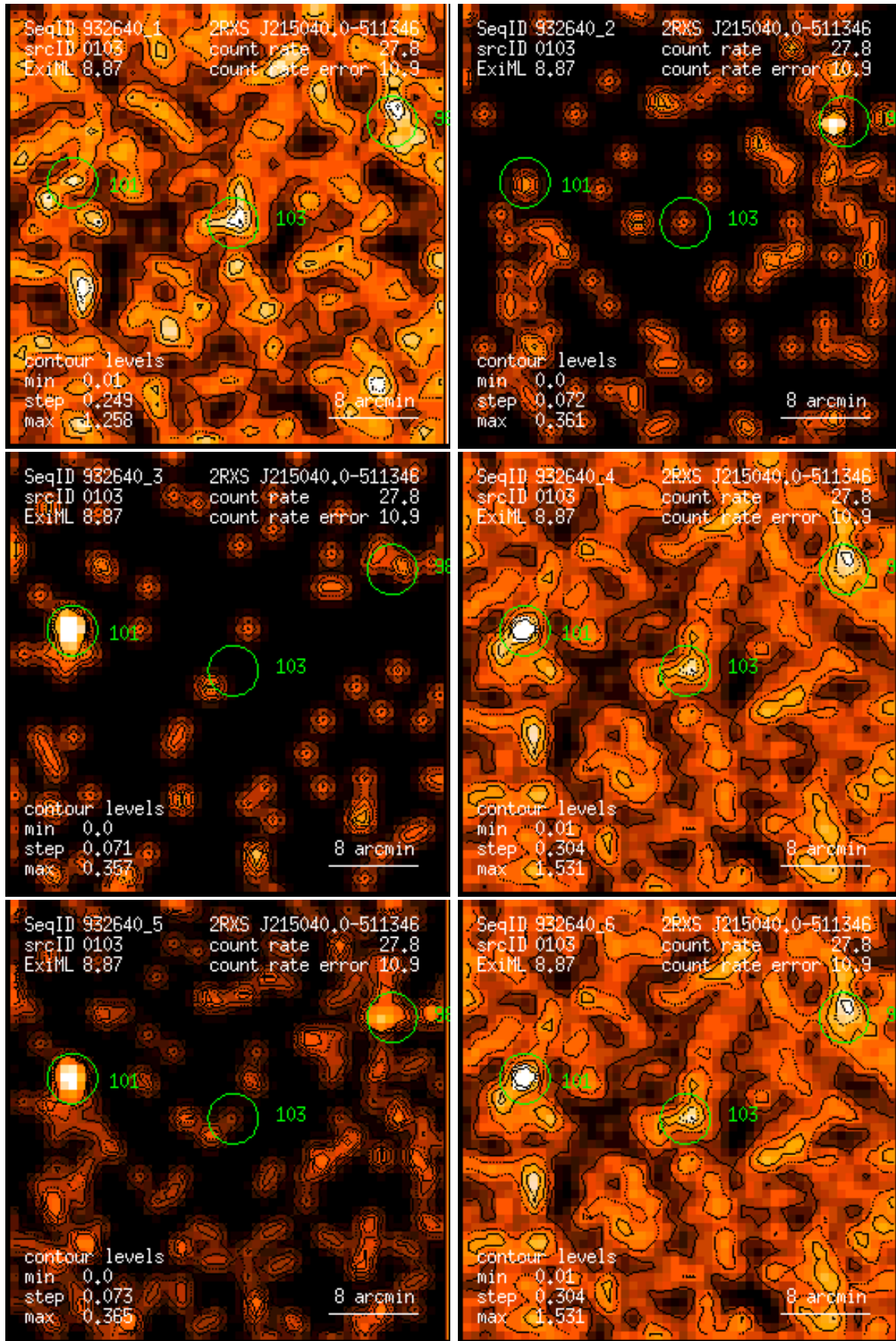
Figure 103: RASS 932640: detection 0103: band rate images, Gaussian filter: (1) PSPC channels 11 – 41, (2) 52 – 90, (3) 91 – 201, (4) 11 – 235, (5) 52 – 201, (6) 11 – 201. Broad band rates in counts/ks. Band rate contour levels in counts/ks/arcmin 2 .
