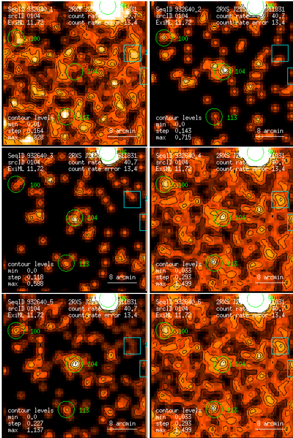
Figure 104: RASS 932640: detection 0104: band rate images, Gaussian filter: (1) PSPC channels 11 – 41, (2) 52 – 90, (3) 91 – 201, (4) 11 – 235, (5) 52 – 201, (6) 11 – 201. Broad band rates in counts/ks. Band rate contour levels in counts/ks/arcmin 2 .
