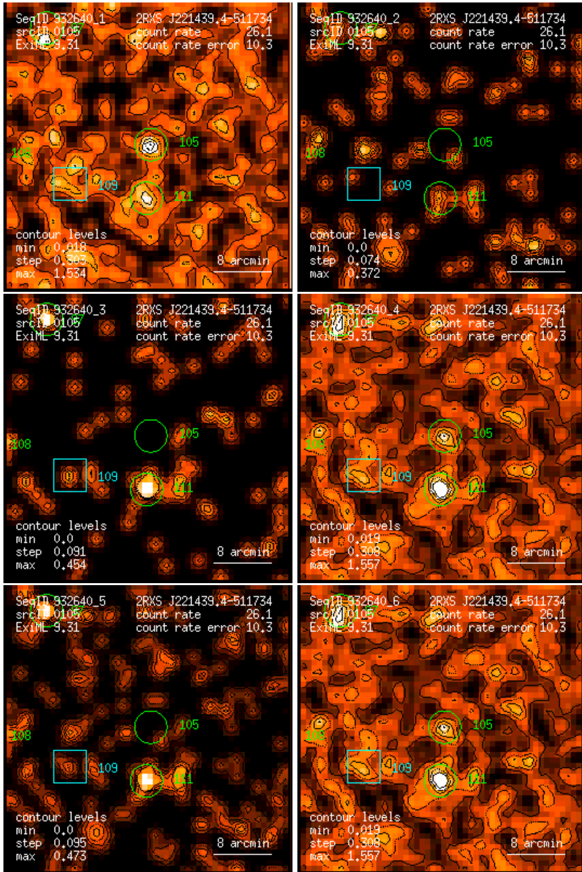
Figure 105: RASS 932640: detection 0105: band rate images, Gaussian filter: (1) PSPC channels 11 – 41, (2) 52 – 90, (3) 91 – 201, (4) 11 – 235, (5) 52 – 201, (6) 11 – 201. Broad band rates in counts/ks. Band rate contour levels in counts/ks/arcmin 2 .
