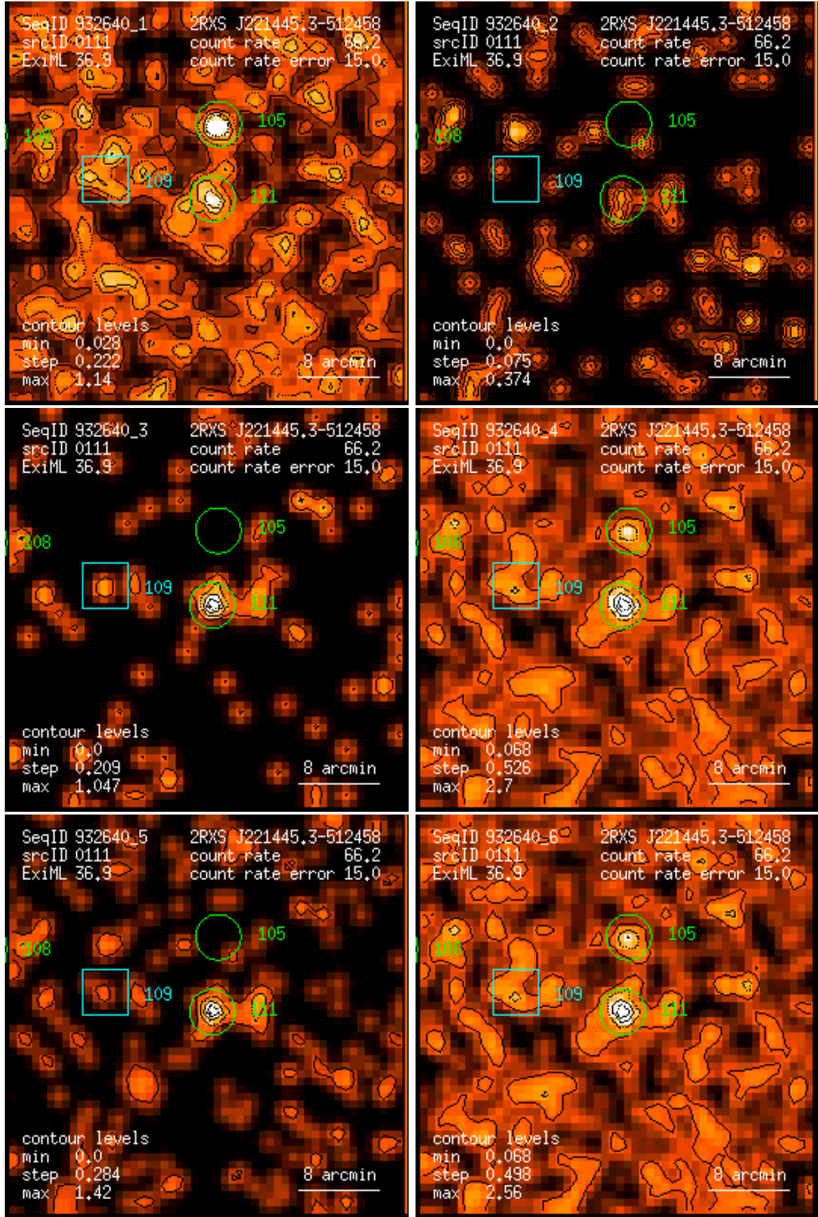
Figure 111: RASS 932640: detection 0111: band rate images, Gaussian filter: (1) PSPC channels 11 – 41, (2) 52 – 90, (3) 91 – 201, (4) 11 – 235, (5) 52 – 201, (6) 11 – 201. Broad band rates in counts/ks. Band rate contour levels in counts/ks/arcmin 2 .
