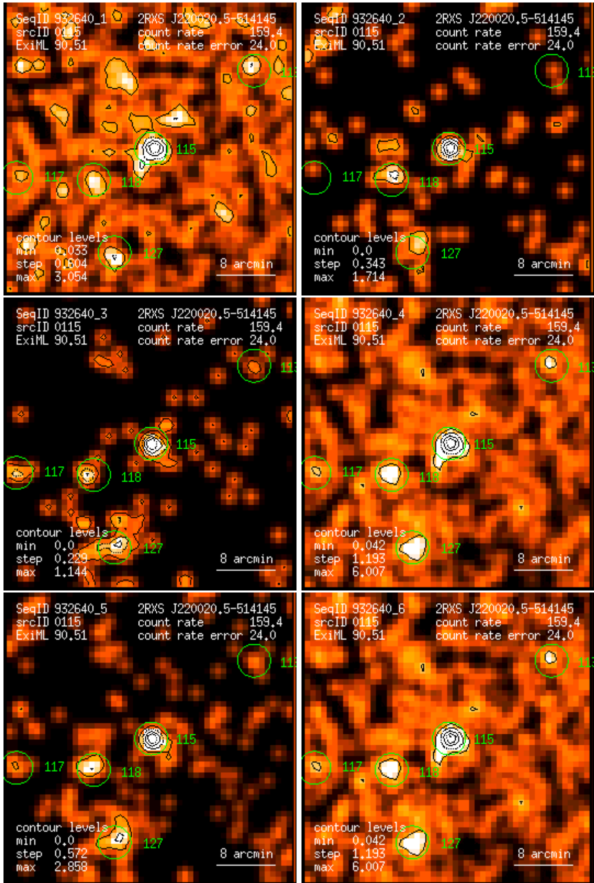
Figure 115: RASS 932640: detection 0115: band rate images, Gaussian filter: (1) PSPC channels 11 – 41, (2) 52 – 90, (3) 91 – 201, (4) 11 – 235, (5) 52 – 201, (6) 11 – 201. Broad band rates in counts/ks. Band rate contour levels in counts/ks/arcmin 2 .
