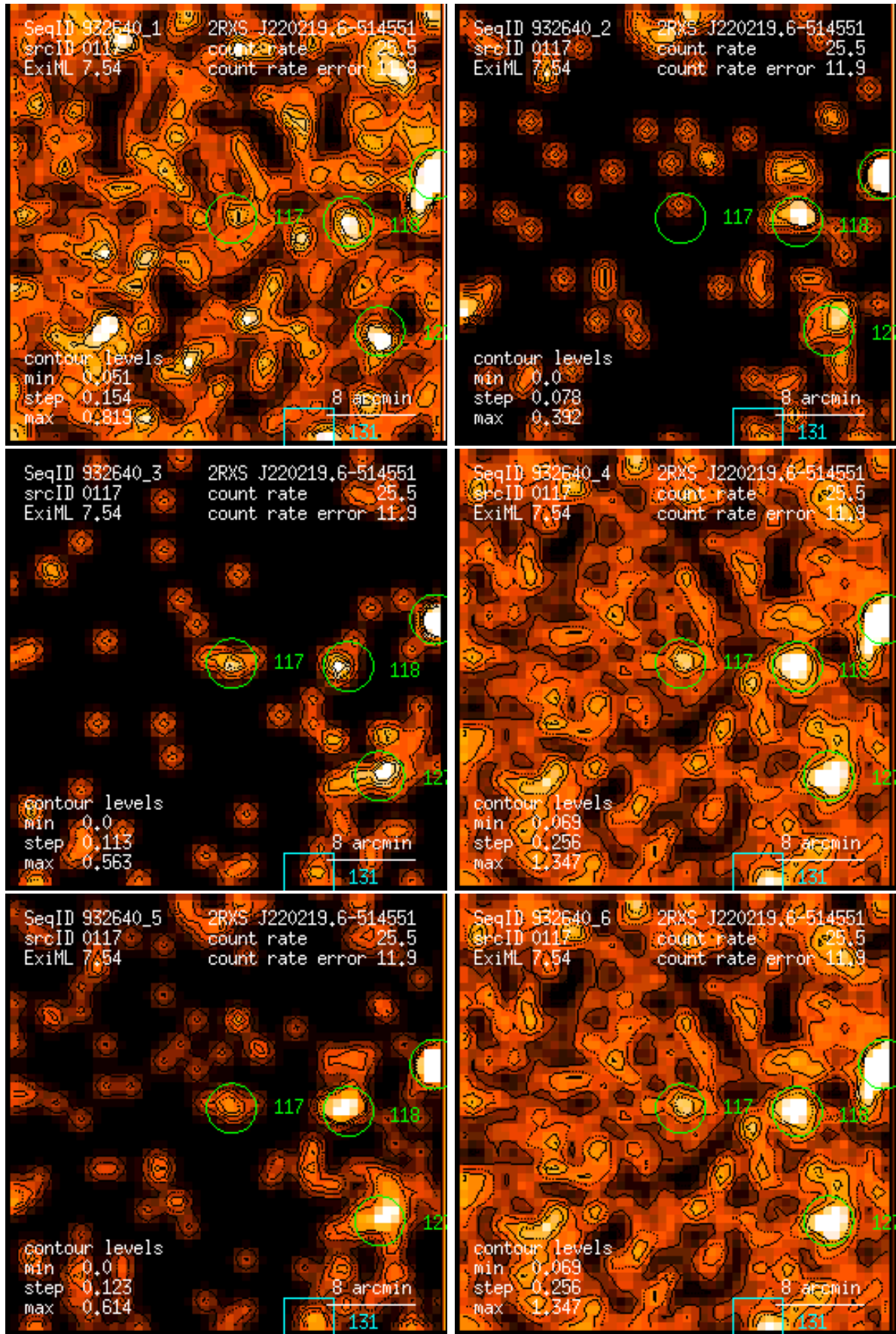
Figure 117: RASS 932640: detection 0117: band rate images, Gaussian filter: (1) PSPC channels 11 – 41, (2) 52 – 90, (3) 91 – 201, (4) 11 – 235, (5) 52 – 201, (6) 11 – 201. Broad band rates in counts/ks. Band rate contour levels in counts/ks/arcmin 2 .
