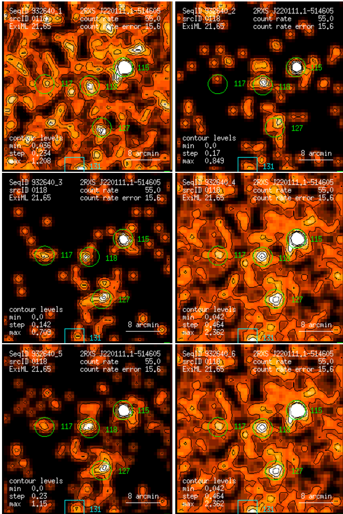
Figure 118: RASS 932640: detection 0118: band rate images, Gaussian filter: (1) PSPC channels 11 – 41, (2) 52 – 90, (3) 91 – 201, (4) 11 – 235, (5) 52 – 201, (6) 11 – 201. Broad band rates in counts/ks. Band rate contour levels in counts/ks/arcmin 2 .
