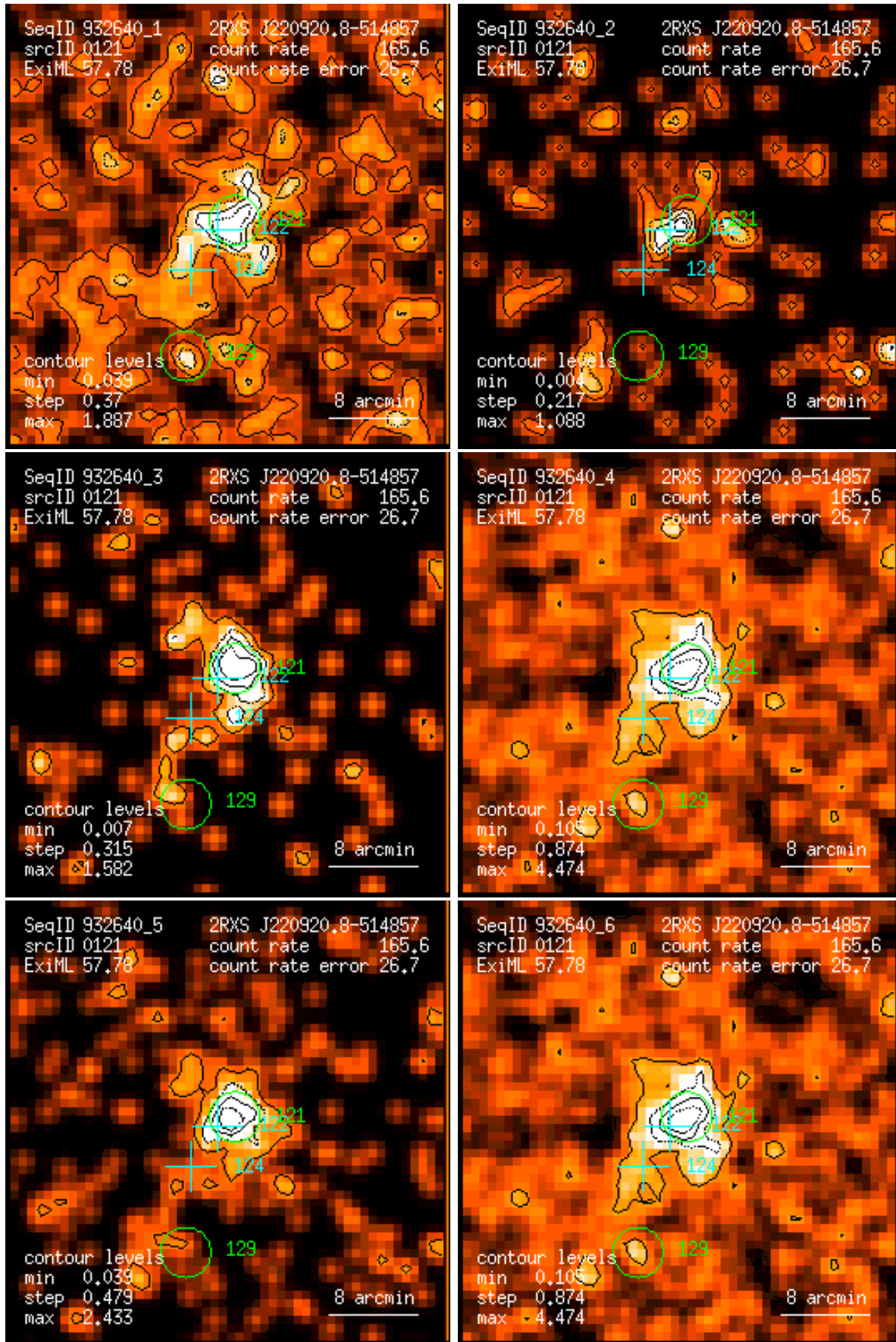
Figure 121: RASS 932640: detection 0121: band rate images, Gaussian filter: (1) PSPC channels 11 – 41, (2) 52 – 90, (3) 91 – 201, (4) 11 – 235, (5) 52 – 201, (6) 11 – 201. Broad band rates in counts/ks. Band rate contour levels in counts/ks/arcmin 2 .
