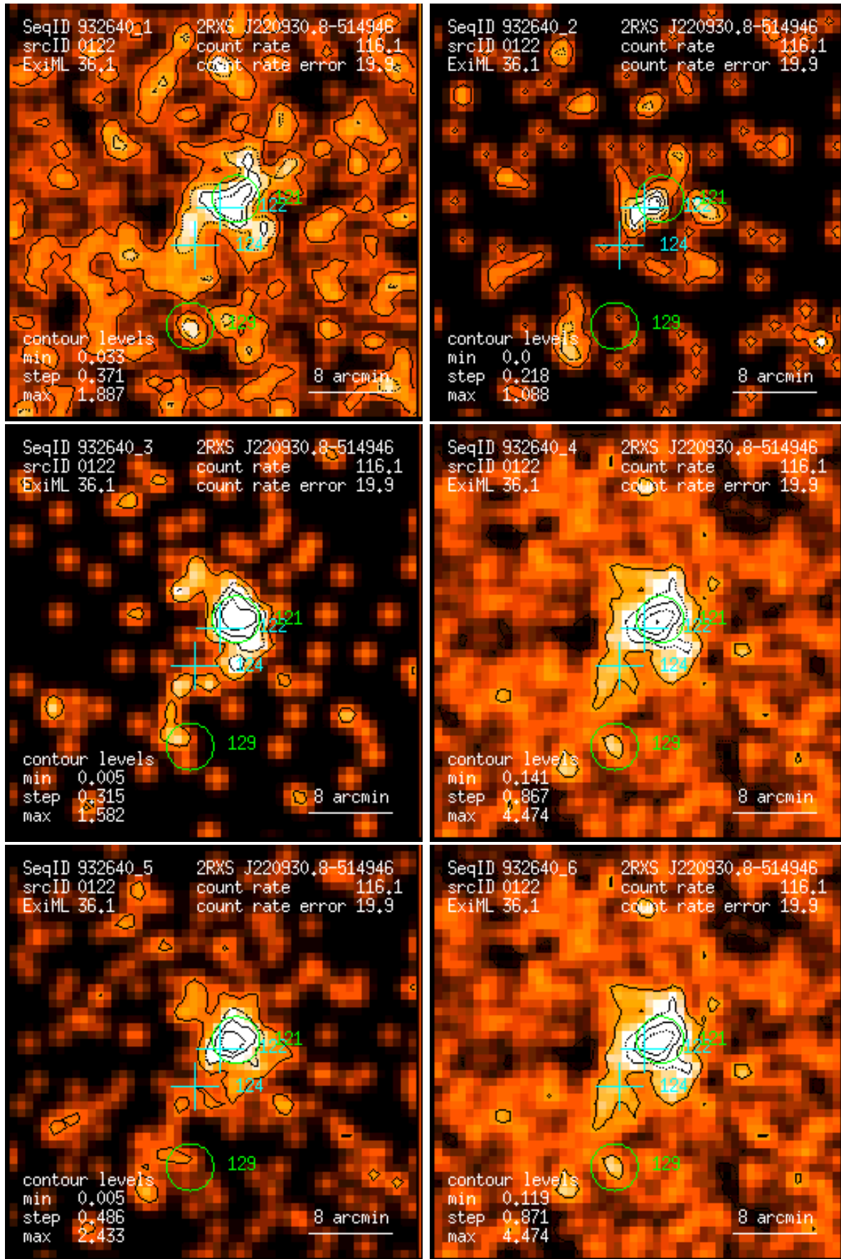
Figure 122: RASS 932640: detection 0122: band rate images, Gaussian filter: (1) PSPC channels 11 – 41, (2) 52 – 90, (3) 91 – 201, (4) 11 – 235, (5) 52 – 201, (6) 11 – 201. Broad band rates in counts/ks. Band rate contour levels in counts/ks/arcmin 2 .
