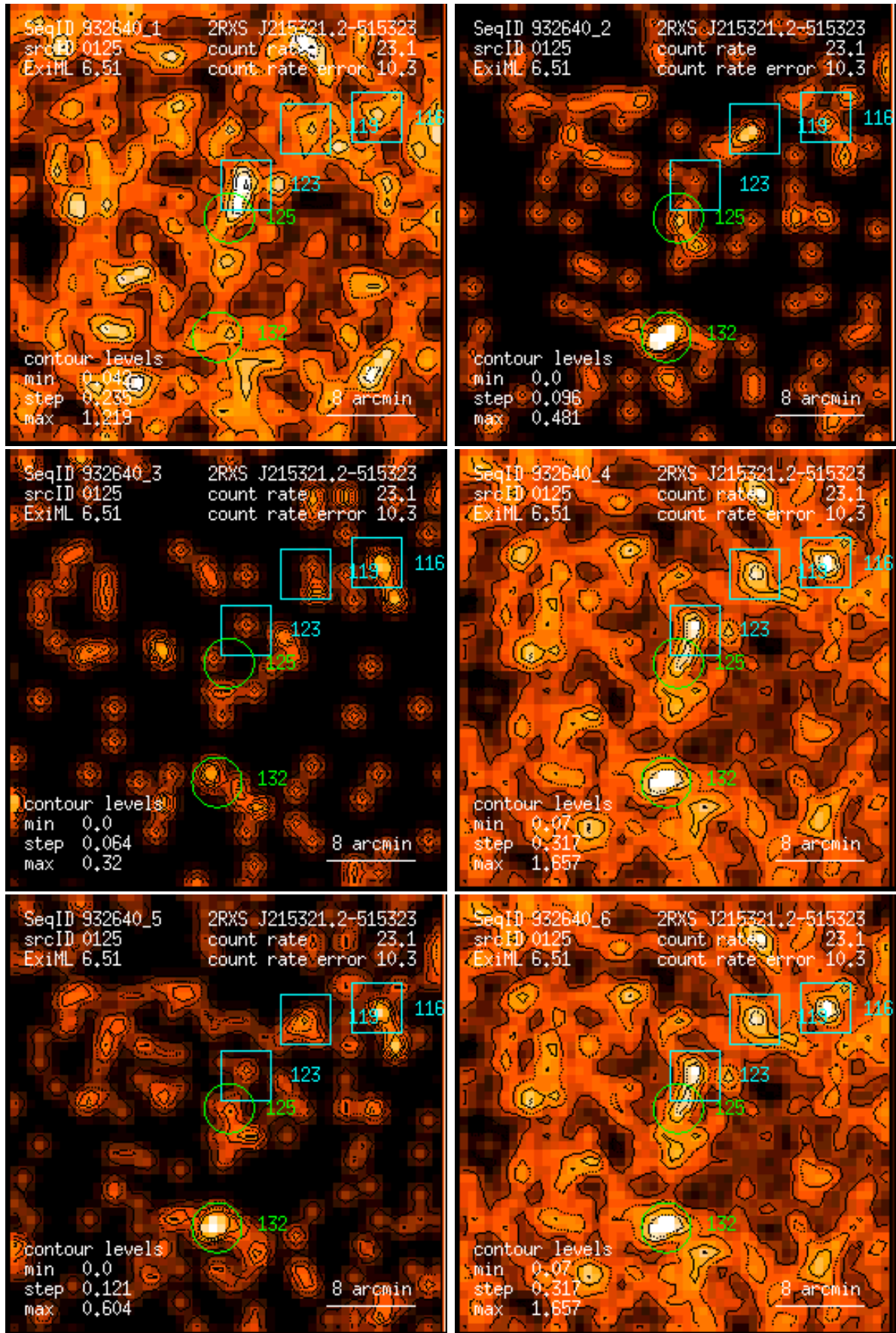
Figure 125: RASS 932640: detection 0125: band rate images, Gaussian filter: (1) PSPC channels 11 – 41, (2) 52 – 90, (3) 91 – 201, (4) 11 – 235, (5) 52 – 201, (6) 11 – 201. Broad band rates in counts/ks. Band rate contour levels in counts/ks/arcmin 2 .
