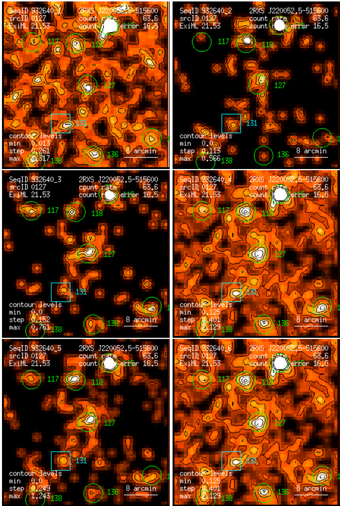
Figure 127: RASS 932640: detection 0127: band rate images, Gaussian filter: (1) PSPC channels 11 – 41, (2) 52 – 90, (3) 91 – 201, (4) 11 – 235, (5) 52 – 201, (6) 11 – 201. Broad band rates in counts/ks. Band rate contour levels in counts/ks/arcmin 2 .
