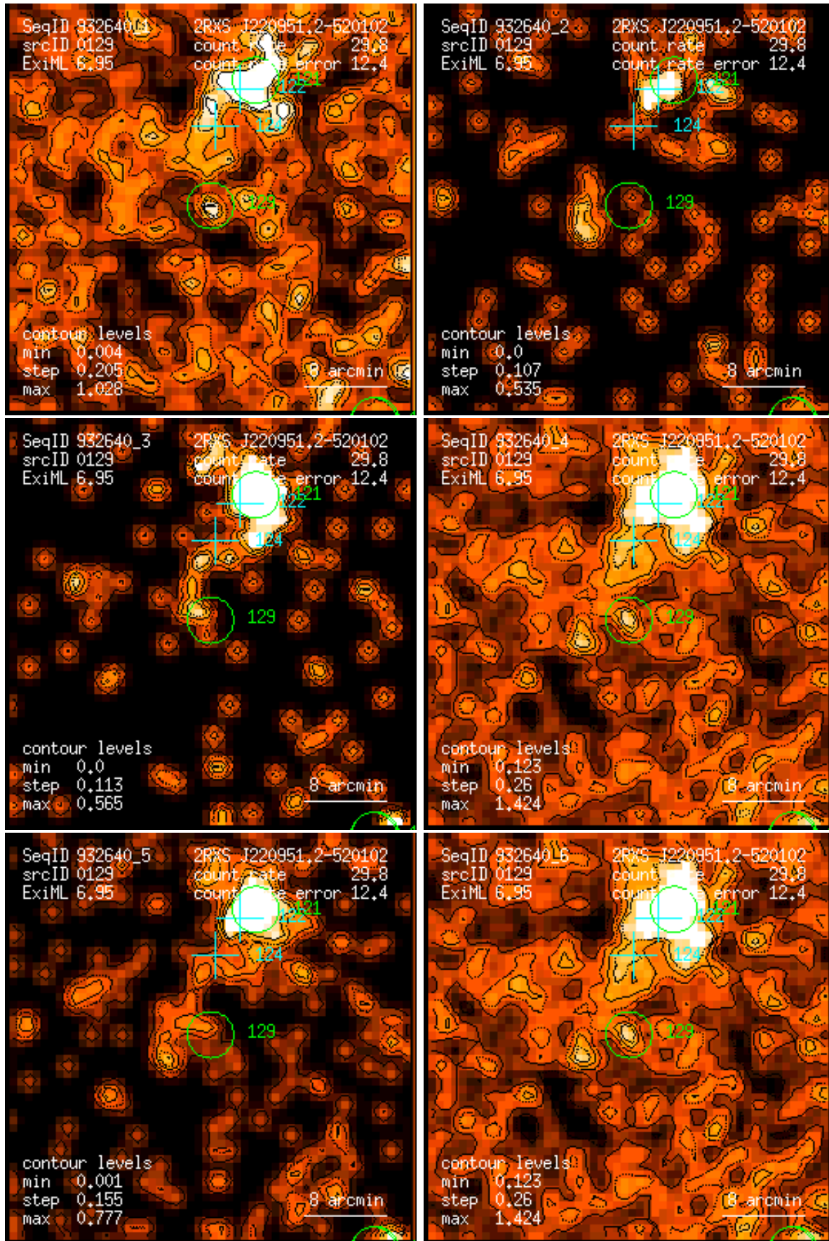
Figure 129: RASS 932640: detection 0129: band rate images, Gaussian filter: (1) PSPC channels 11 – 41, (2) 52 – 90, (3) 91 – 201, (4) 11 – 235, (5) 52 – 201, (6) 11 – 201. Broad band rates in counts/ks. Band rate contour levels in counts/ks/arcmin 2 .
