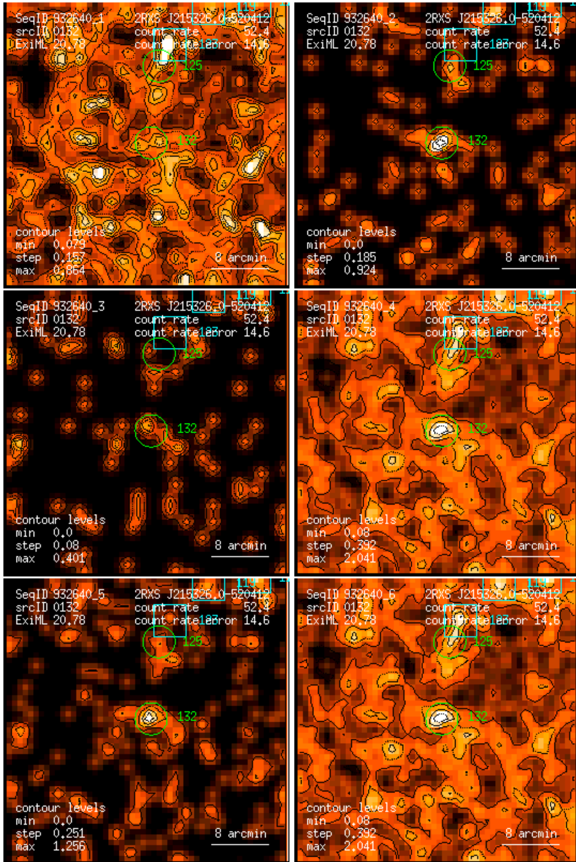
Figure 132: RASS 932640: detection 0132: band rate images, Gaussian filter: (1) PSPC channels 11 – 41, (2) 52 – 90, (3) 91 – 201, (4) 11 – 235, (5) 52 – 201, (6) 11 – 201. Broad band rates in counts/ks. Band rate contour levels in counts/ks/arcmin 2 .
