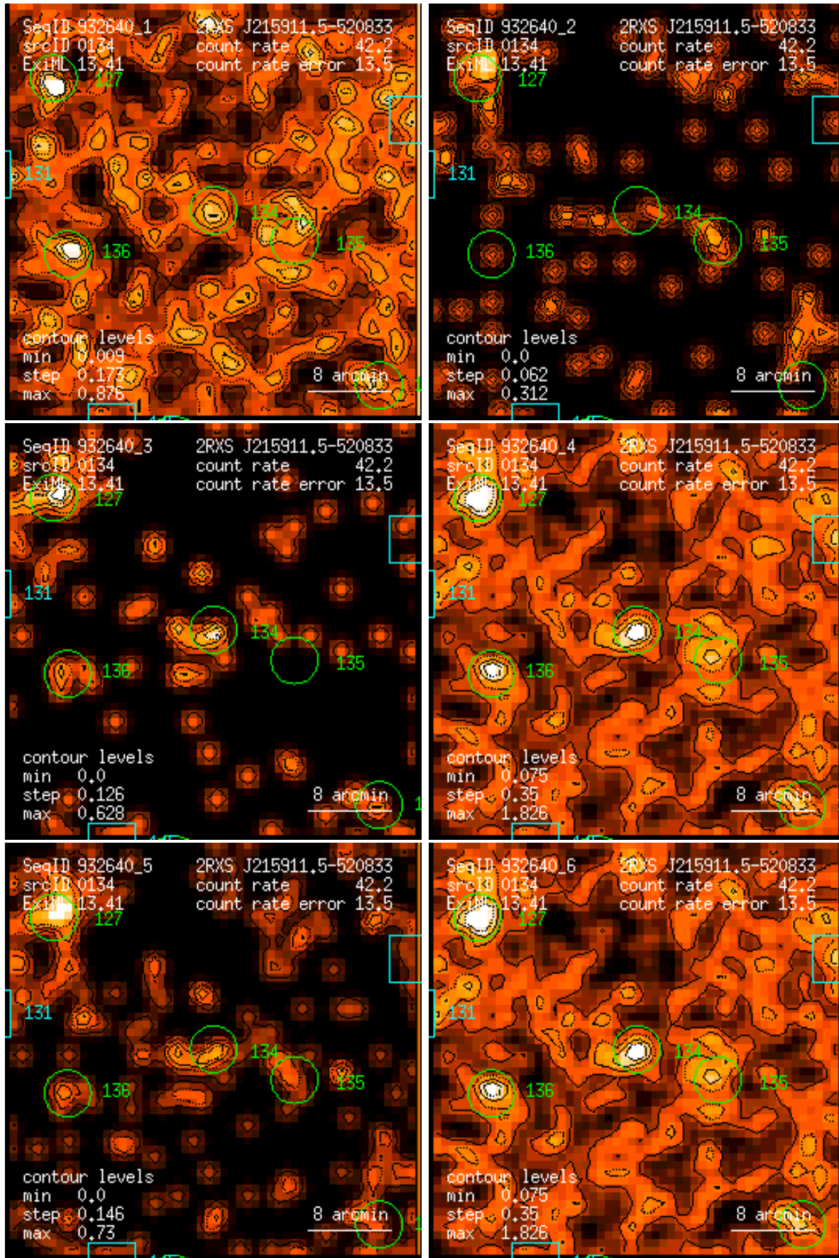
Figure 134: RASS 932640: detection 0134: band rate images, Gaussian filter: (1) PSPC channels 11 – 41, (2) 52 – 90, (3) 91 – 201, (4) 11 – 235, (5) 52 – 201, (6) 11 – 201. Broad band rates in counts/ks. Band rate contour levels in counts/ks/arcmin 2 .
