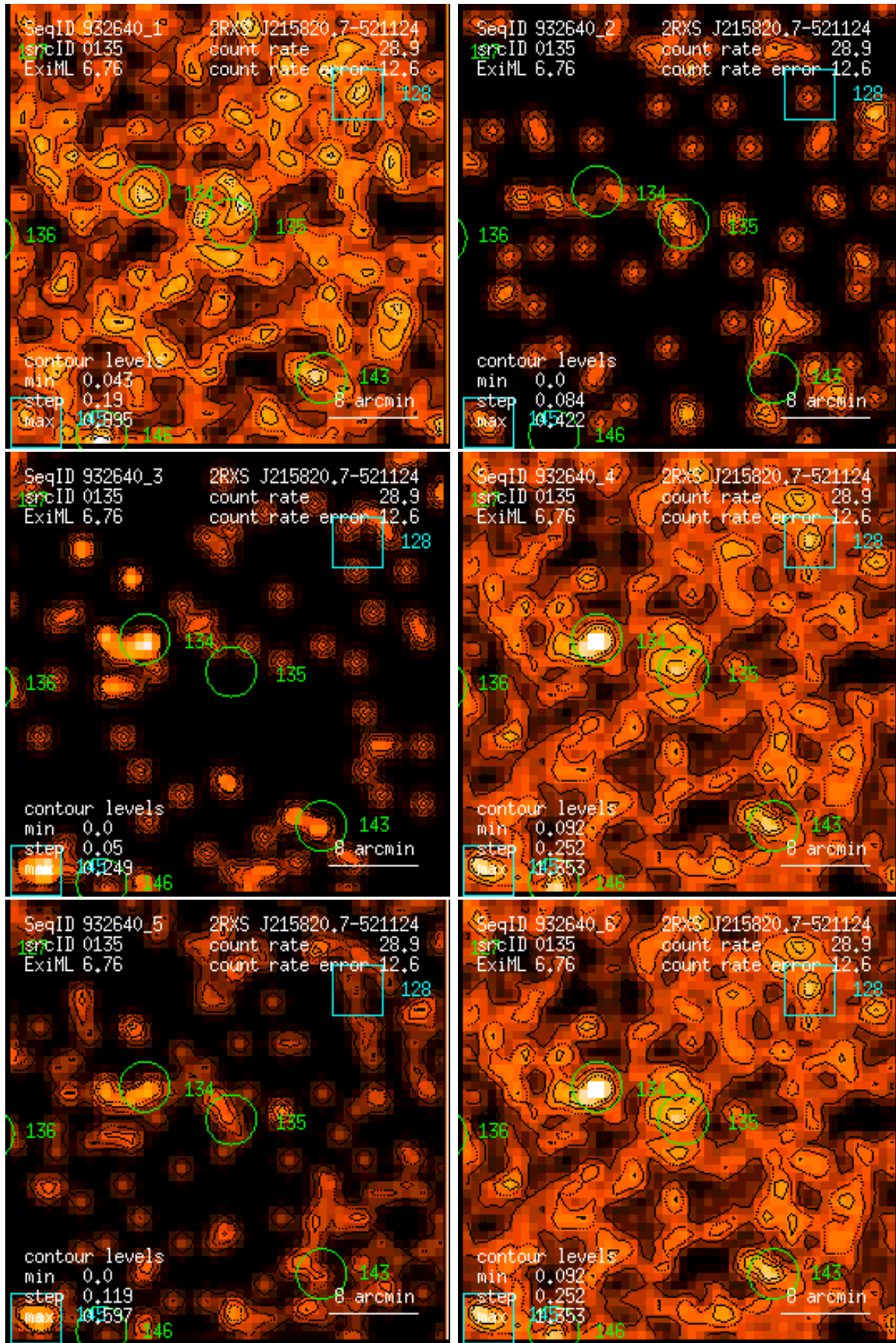
Figure 135: RASS 932640: detection 0135: band rate images, Gaussian filter: (1) PSPC channels 11 – 41, (2) 52 – 90, (3) 91 – 201, (4) 11 – 235, (5) 52 – 201, (6) 11 – 201. Broad band rates in counts/ks. Band rate contour levels in counts/ks/arcmin 2 .
