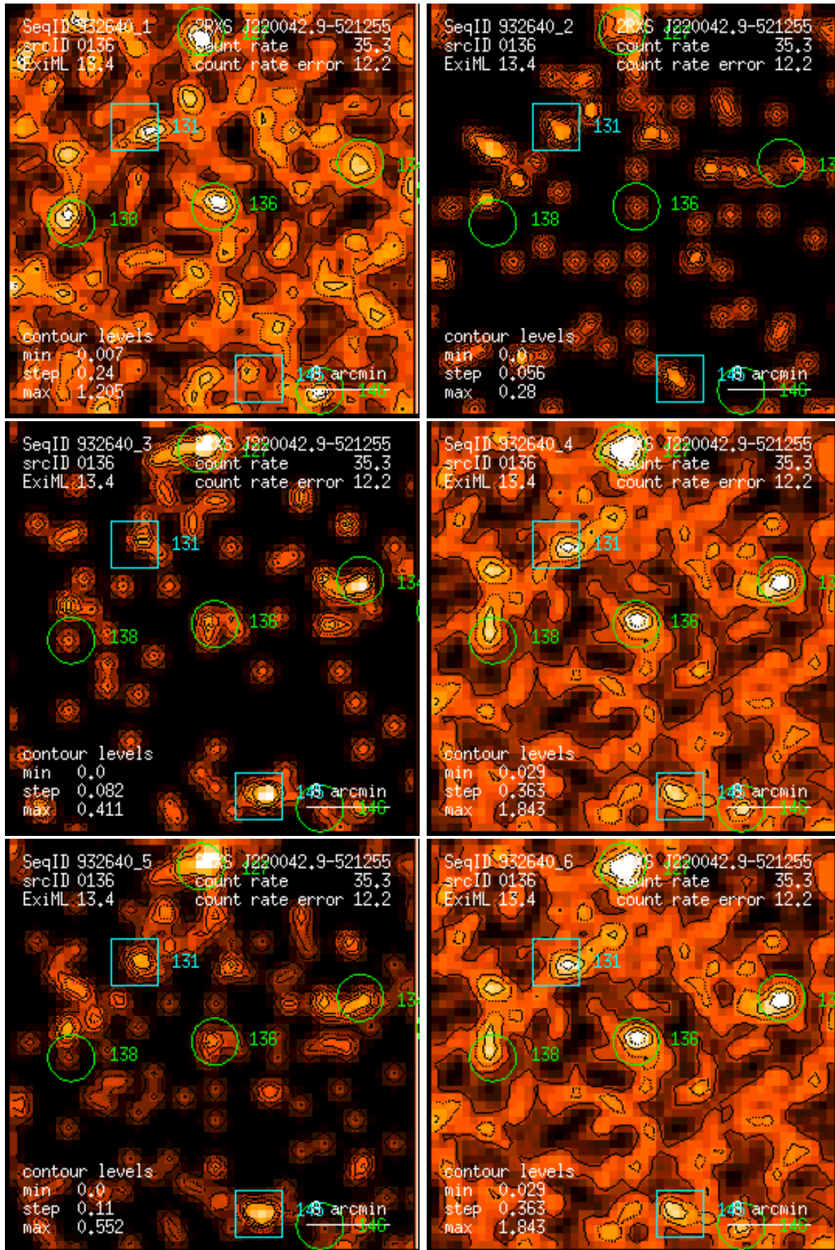
Figure 136: RASS 932640: detection 0136: band rate images, Gaussian filter: (1) PSPC channels 11 – 41, (2) 52 – 90, (3) 91 – 201, (4) 11 – 235, (5) 52 – 201, (6) 11 – 201. Broad band rates in counts/ks. Band rate contour levels in counts/ks/arcmin 2 .
