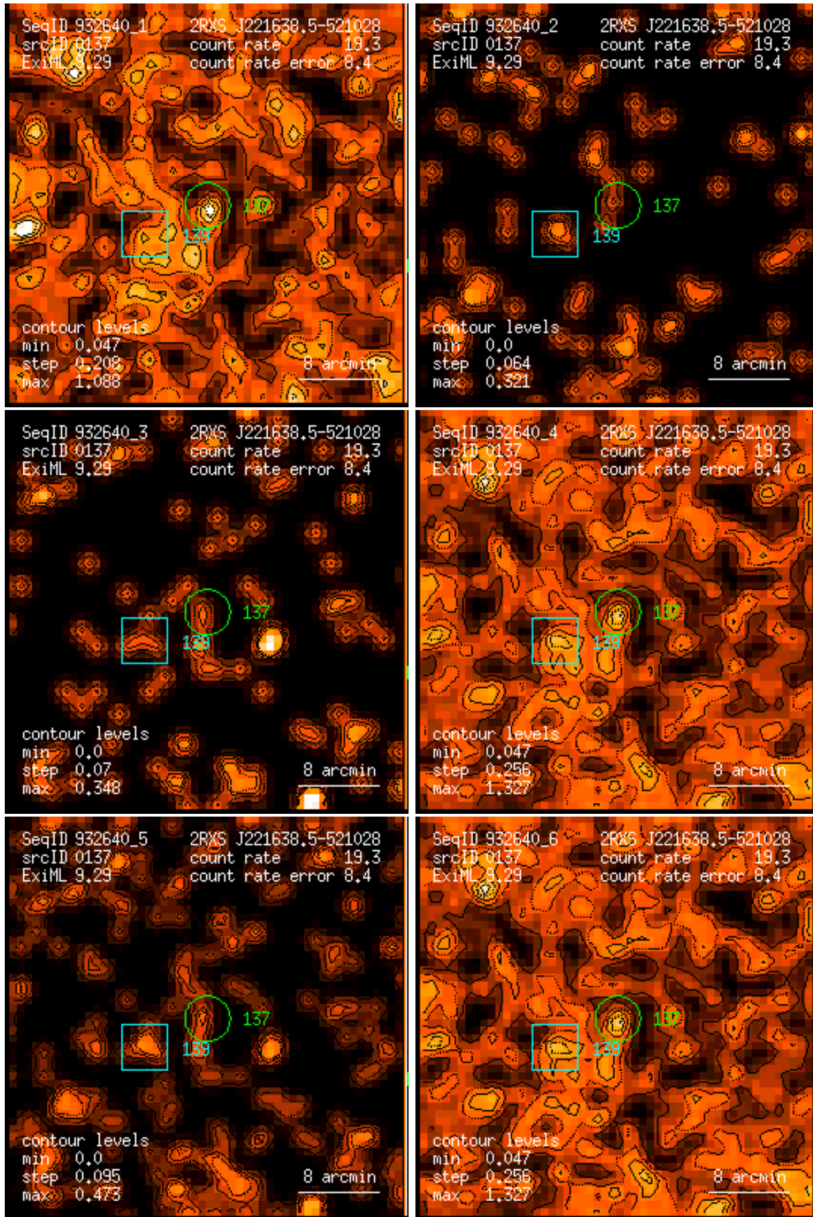
Figure 137: RASS 932640: detection 0137: band rate images, Gaussian filter: (1) PSPC channels 11 – 41, (2) 52 – 90, (3) 91 – 201, (4) 11 – 235, (5) 52 – 201, (6) 11 – 201. Broad band rates in counts/ks. Band rate contour levels in counts/ks/arcmin 2 .
