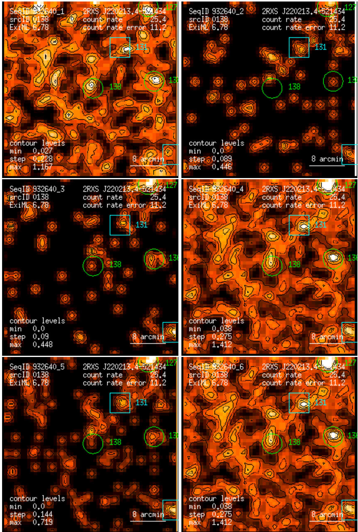
Figure 138: RASS 932640: detection 0138: band rate images, Gaussian filter: (1) PSPC channels 11 – 41, (2) 52 – 90, (3) 91 – 201, (4) 11 – 235, (5) 52 – 201, (6) 11 – 201. Broad band rates in counts/ks. Band rate contour levels in counts/ks/arcmin 2 .
