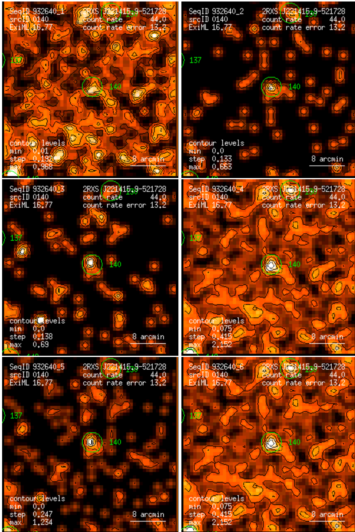
Figure 140: RASS 932640: detection 0140: band rate images, Gaussian filter: (1) PSPC channels 11 – 41, (2) 52 – 90, (3) 91 – 201, (4) 11 – 235, (5) 52 – 201, (6) 11 – 201. Broad band rates in counts/ks. Band rate contour levels in counts/ks/arcmin 2 .
