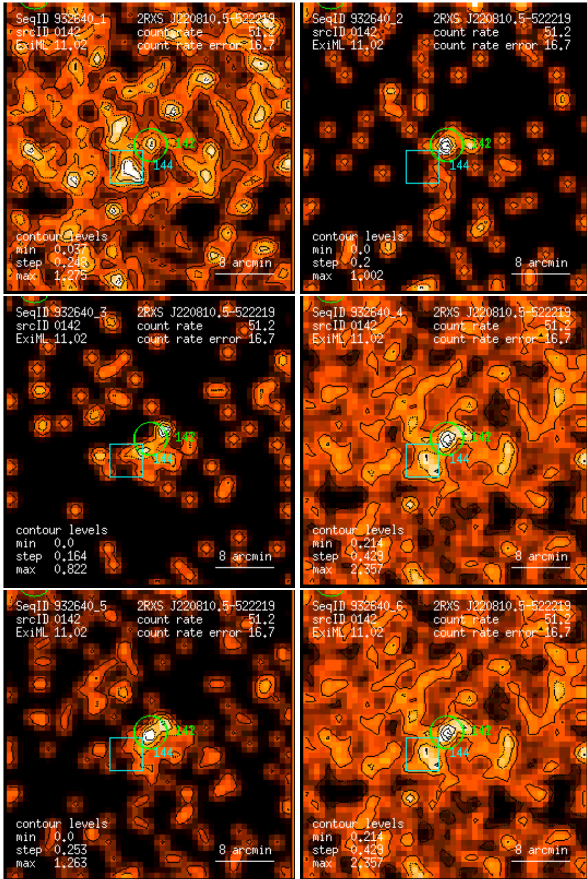
Figure 142: RASS 932640: detection 0142: band rate images, Gaussian filter: (1) PSPC channels 11 – 41, (2) 52 – 90, (3) 91 – 201, (4) 11 – 235, (5) 52 – 201, (6) 11 – 201. Broad band rates in counts/ks. Band rate contour levels in counts/ks/arcmin 2 .
