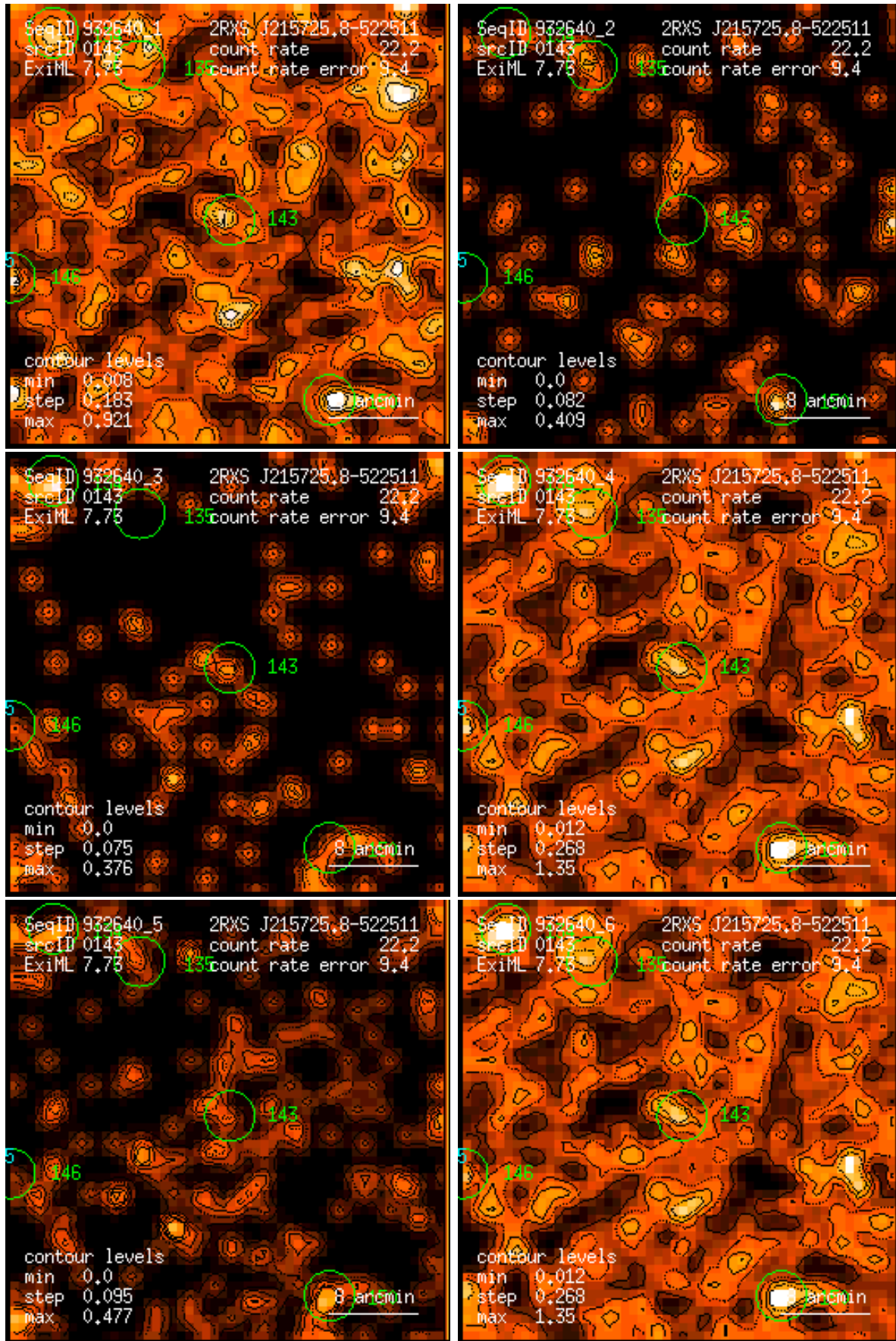
Figure 143: RASS 932640: detection 0143: band rate images, Gaussian filter: (1) PSPC channels 11 – 41, (2) 52 – 90, (3) 91 – 201, (4) 11 – 235, (5) 52 – 201, (6) 11 – 201. Broad band rates in counts/ks. Band rate contour levels in counts/ks/arcmin 2 .
