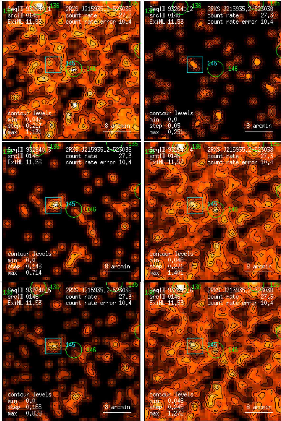
Figure 146: RASS 932640: detection 0146: band rate images, Gaussian filter: (1) PSPC channels 11 – 41, (2) 52 – 90, (3) 91 – 201, (4) 11 – 235, (5) 52 – 201, (6) 11 – 201. Broad band rates in counts/ks. Band rate contour levels in counts/ks/arcmin 2 .
