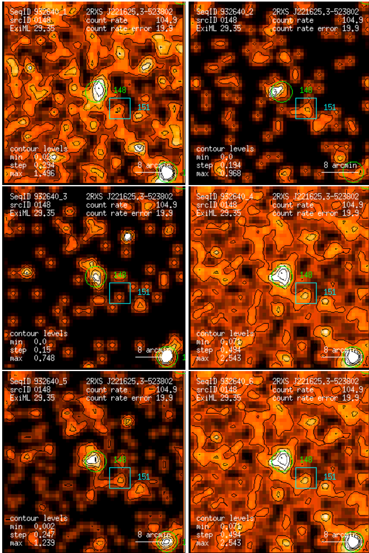
Figure 148: RASS 932640: detection 0148: band rate images, Gaussian filter: (1) PSPC channels 11 – 41, (2) 52 – 90, (3) 91 – 201, (4) 11 – 235, (5) 52 – 201, (6) 11 – 201. Broad band rates in counts/ks. Band rate contour levels in counts/ks/arcmin 2 .
