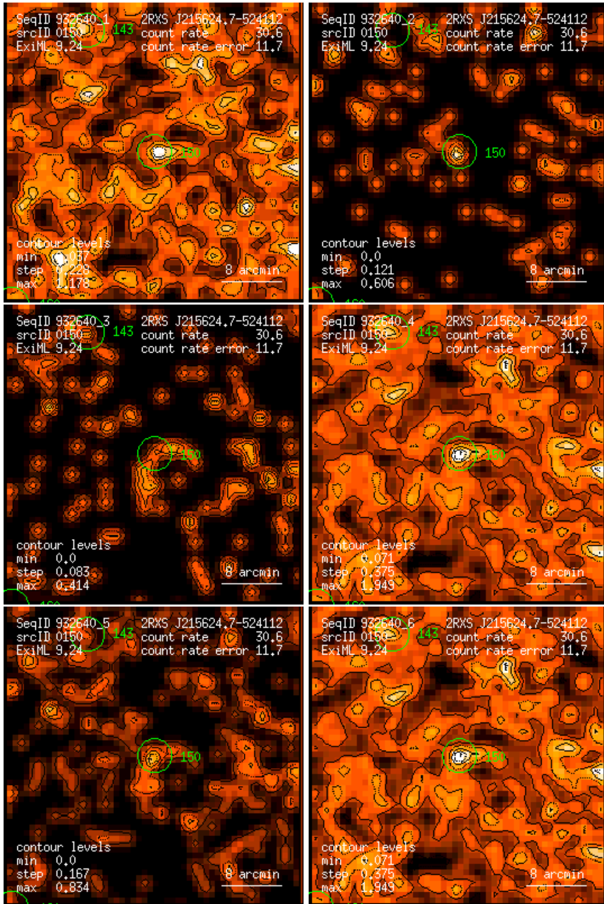
Figure 150: RASS 932640: detection 0150: band rate images, Gaussian filter: (1) PSPC channels 11 – 41, (2) 52 – 90, (3) 91 – 201, (4) 11 – 235, (5) 52 – 201, (6) 11 – 201. Broad band rates in counts/ks. Band rate contour levels in counts/ks/arcmin 2 .
