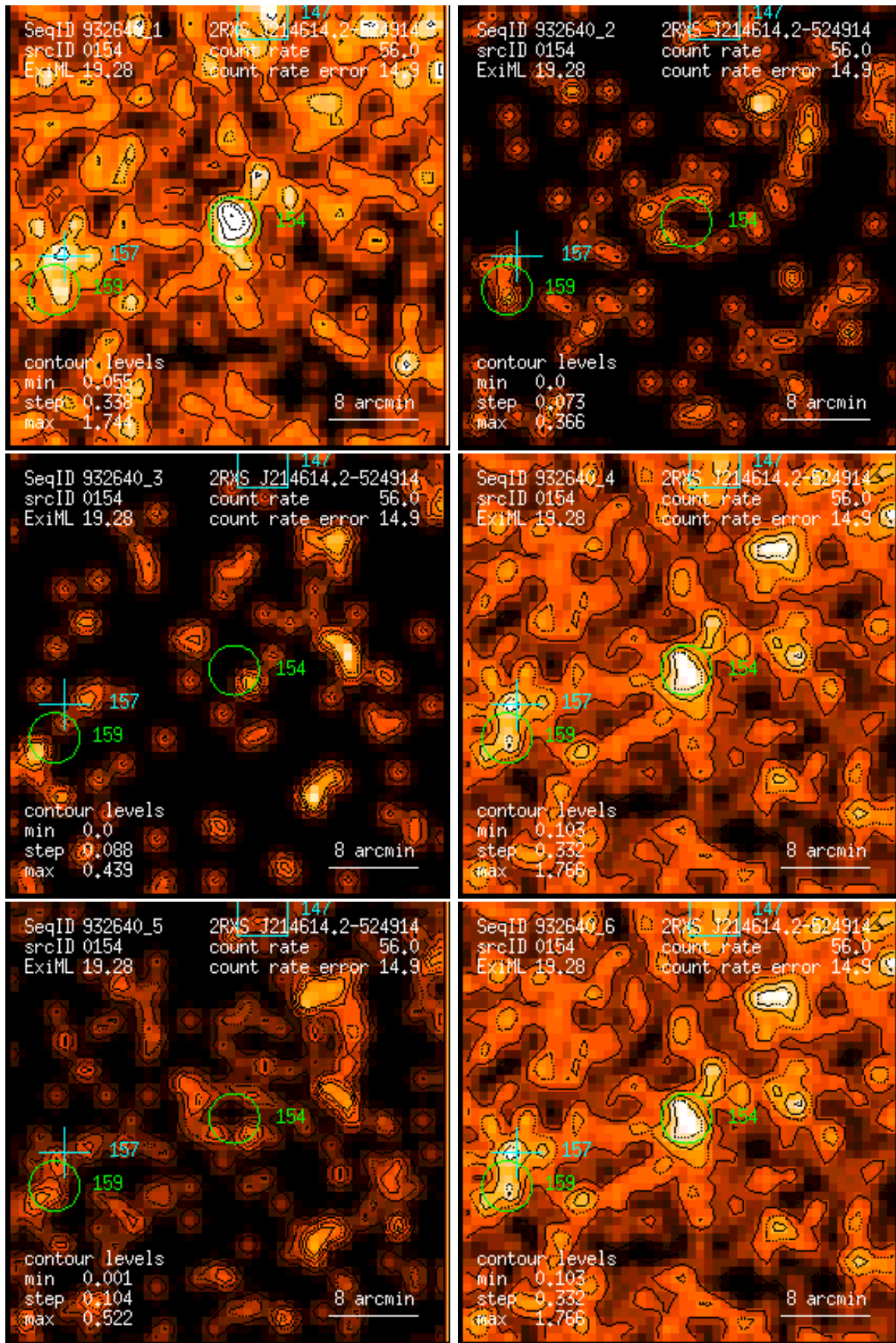
Figure 154: RASS 932640: detection 0154: band rate images, Gaussian filter: (1) PSPC channels 11 – 41, (2) 52 – 90, (3) 91 – 201, (4) 11 – 235, (5) 52 – 201, (6) 11 – 201. Broad band rates in counts/ks. Band rate contour levels in counts/ks/arcmin 2 .
