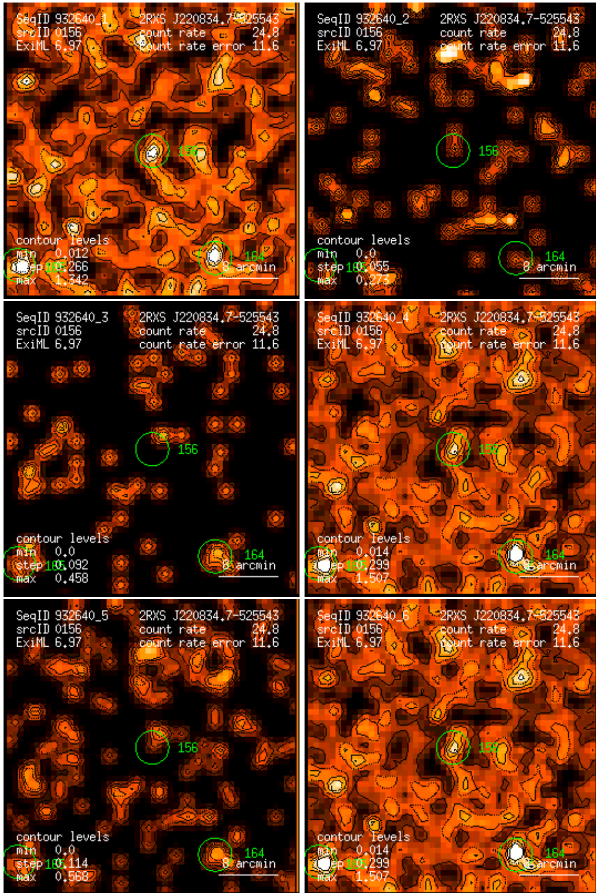
Figure 156: RASS 932640: detection 0156: band rate images, Gaussian filter: (1) PSPC channels 11 – 41, (2) 52 – 90, (3) 91 – 201, (4) 11 – 235, (5) 52 – 201, (6) 11 – 201. Broad band rates in counts/ks. Band rate contour levels in counts/ks/arcmin 2 .
