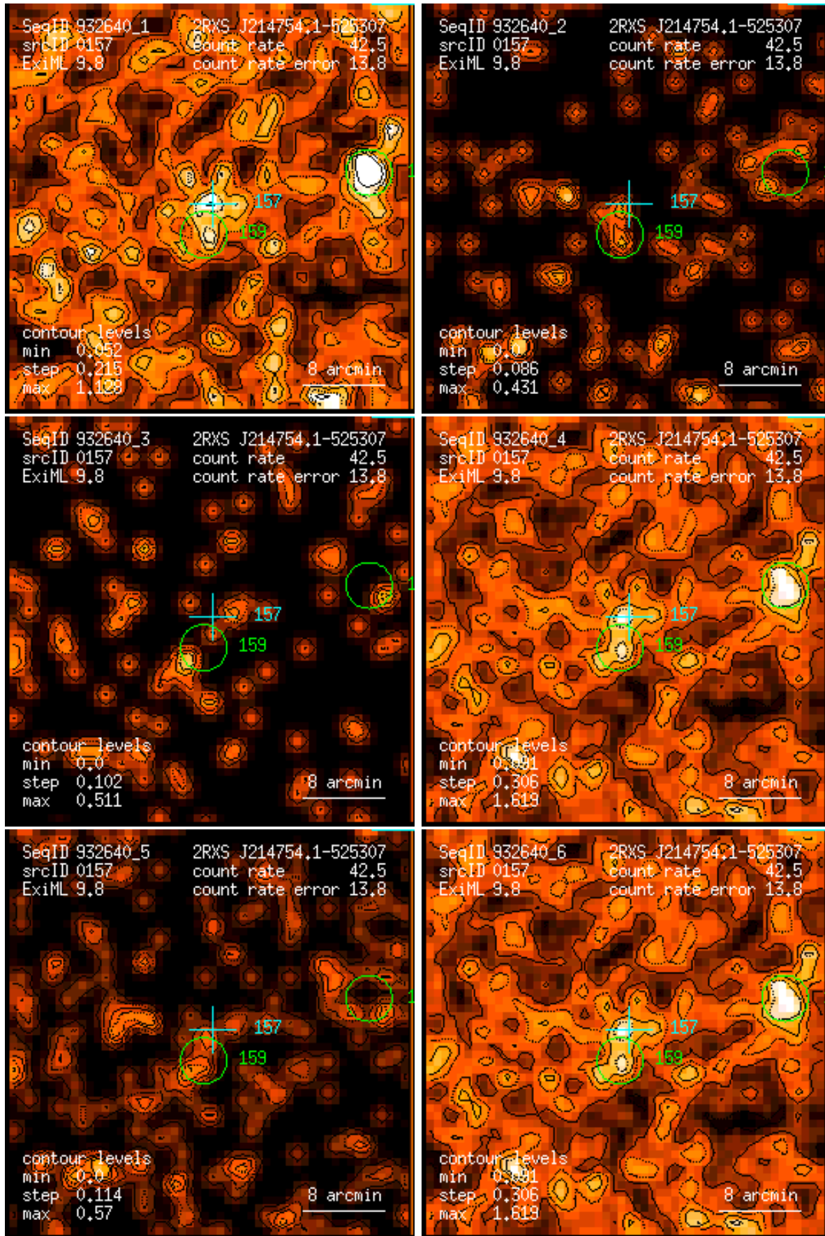
Figure 157: RASS 932640: detection 0157: band rate images, Gaussian filter: (1) PSPC channels 11 – 41, (2) 52 – 90, (3) 91 – 201, (4) 11 – 235, (5) 52 – 201, (6) 11 – 201. Broad band rates in counts/ks. Band rate contour levels in counts/ks/arcmin 2 .
