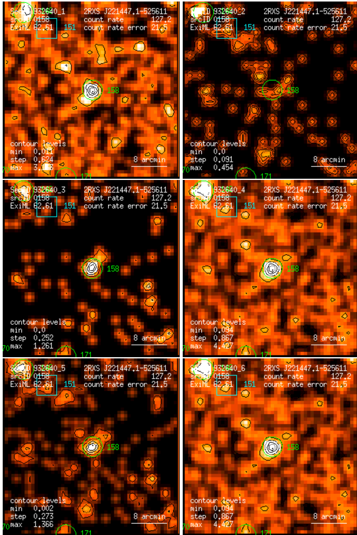
Figure 158: RASS 932640: detection 0158: band rate images, Gaussian filter: (1) PSPC channels 11 – 41, (2) 52 – 90, (3) 91 – 201, (4) 11 – 235, (5) 52 – 201, (6) 11 – 201. Broad band rates in counts/ks. Band rate contour levels in counts/ks/arcmin 2 .
