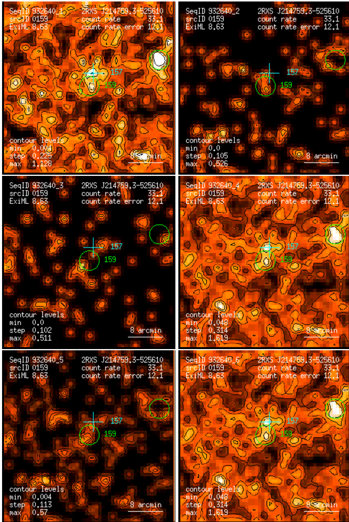
Figure 159: RASS 932640: detection 0159: band rate images, Gaussian filter: (1) PSPC channels 11 – 41, (2) 52 – 90, (3) 91 – 201, (4) 11 – 235, (5) 52 – 201, (6) 11 – 201. Broad band rates in counts/ks. Band rate contour levels in counts/ks/arcmin 2 .
